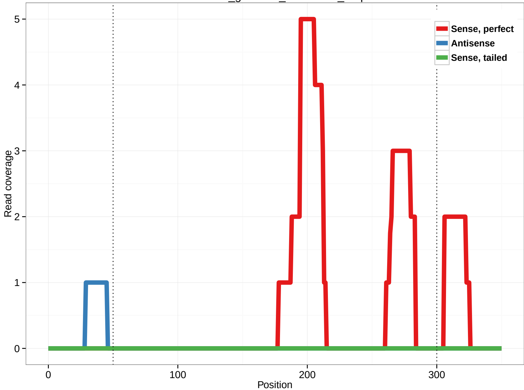
rheMac3_genscan_chr5.2207_7.5p
