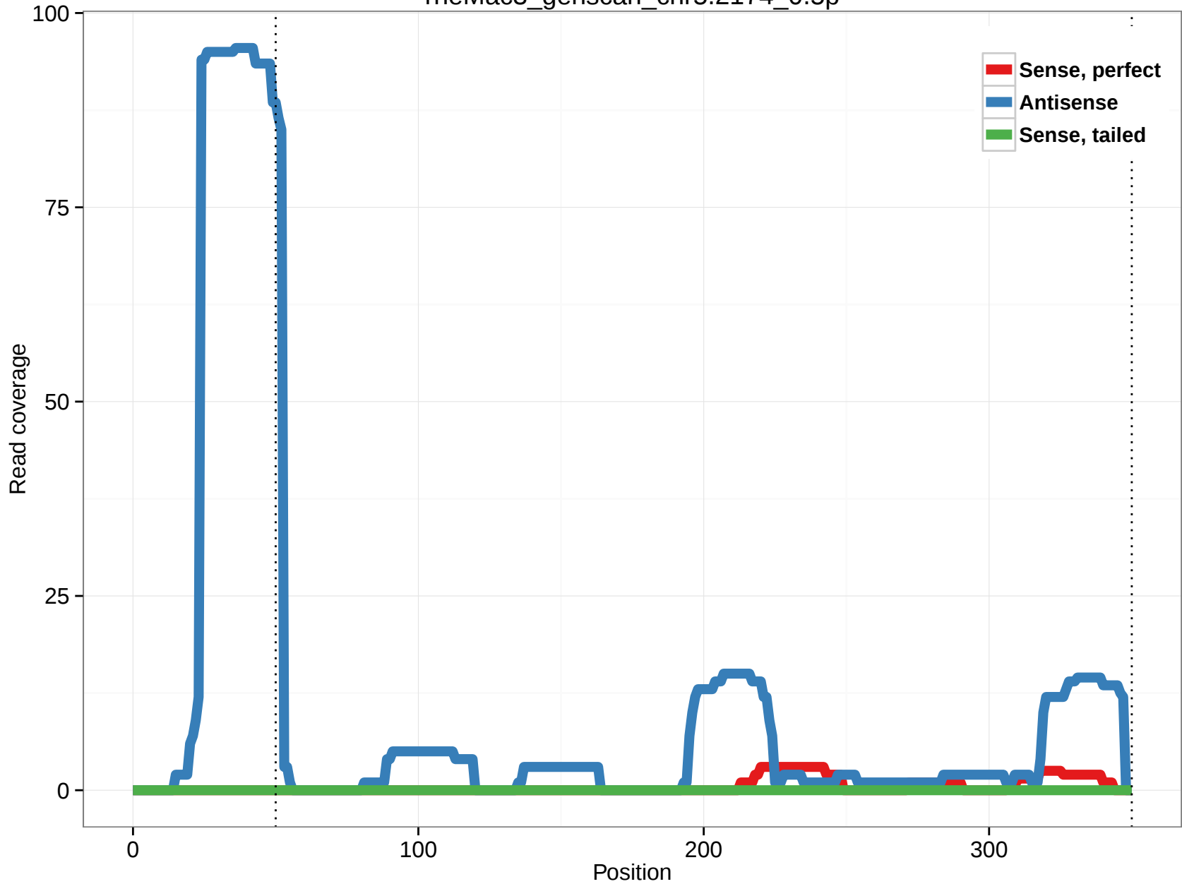
rheMac3_genscan_chr5.2174_0.5p
