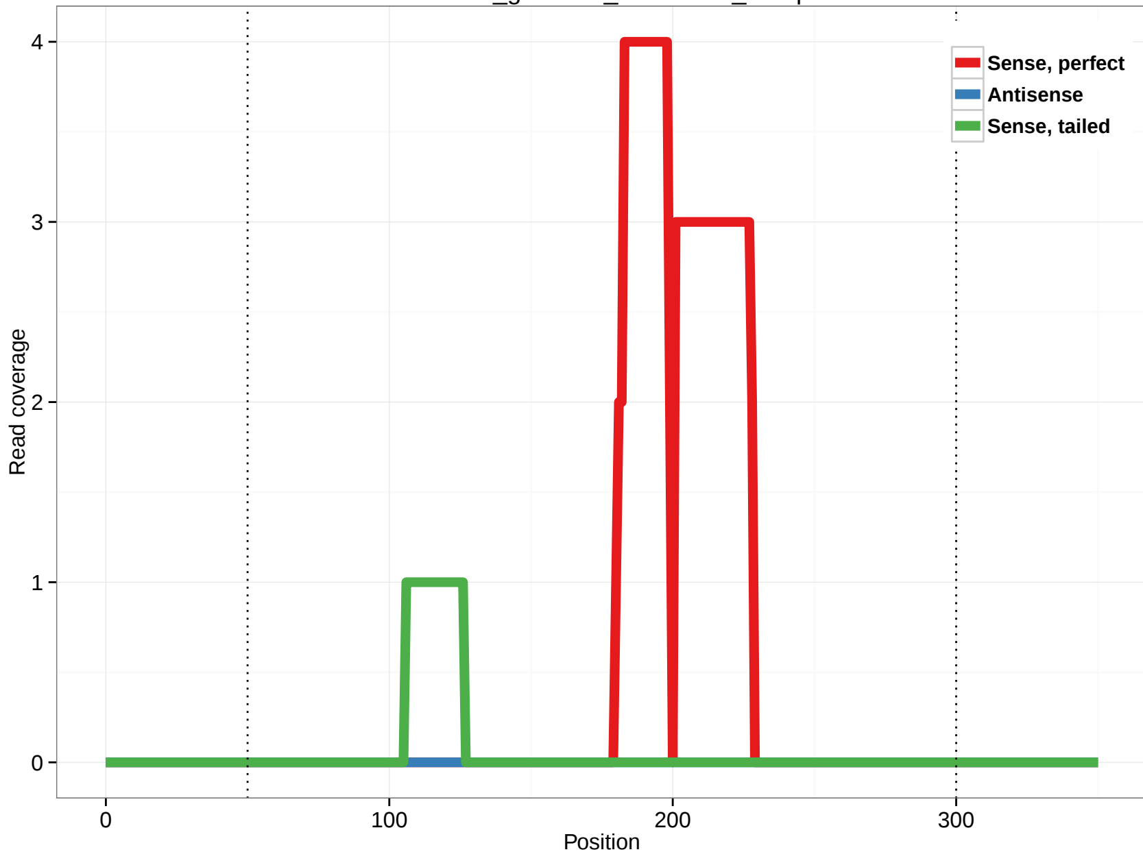
rheMac3_genscan_chr5.2172_14.5p
