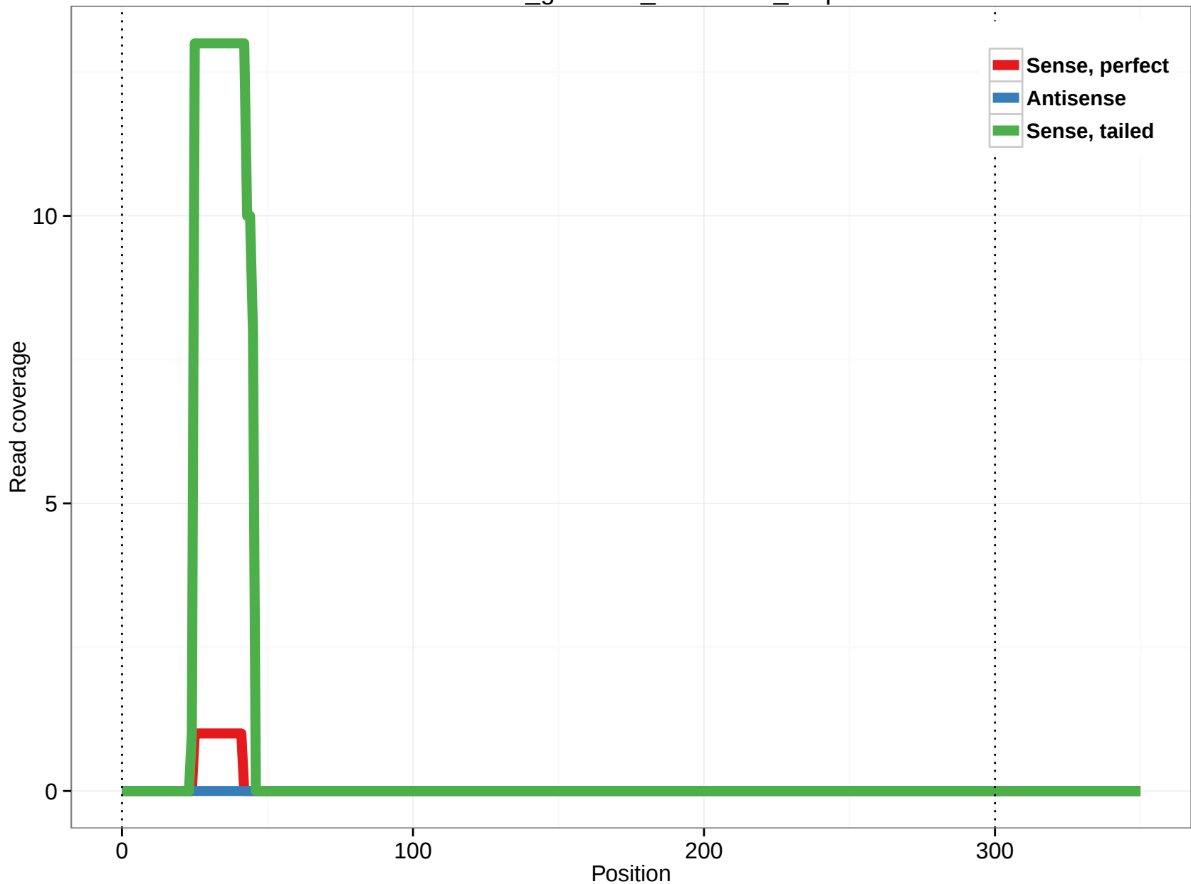
rheMac3_genscan_chr5.2107_5.3p
