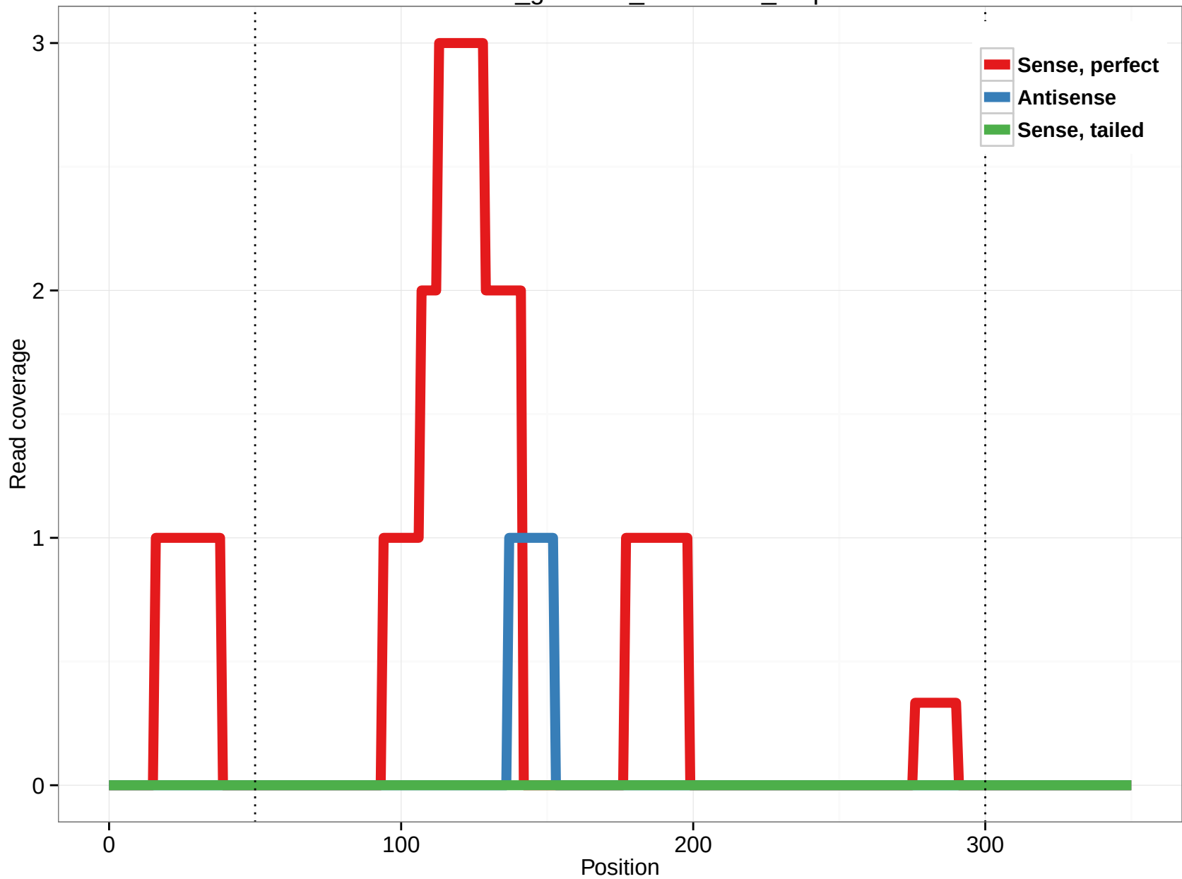
rheMac3_genscan_chr5.2096_8.5p
