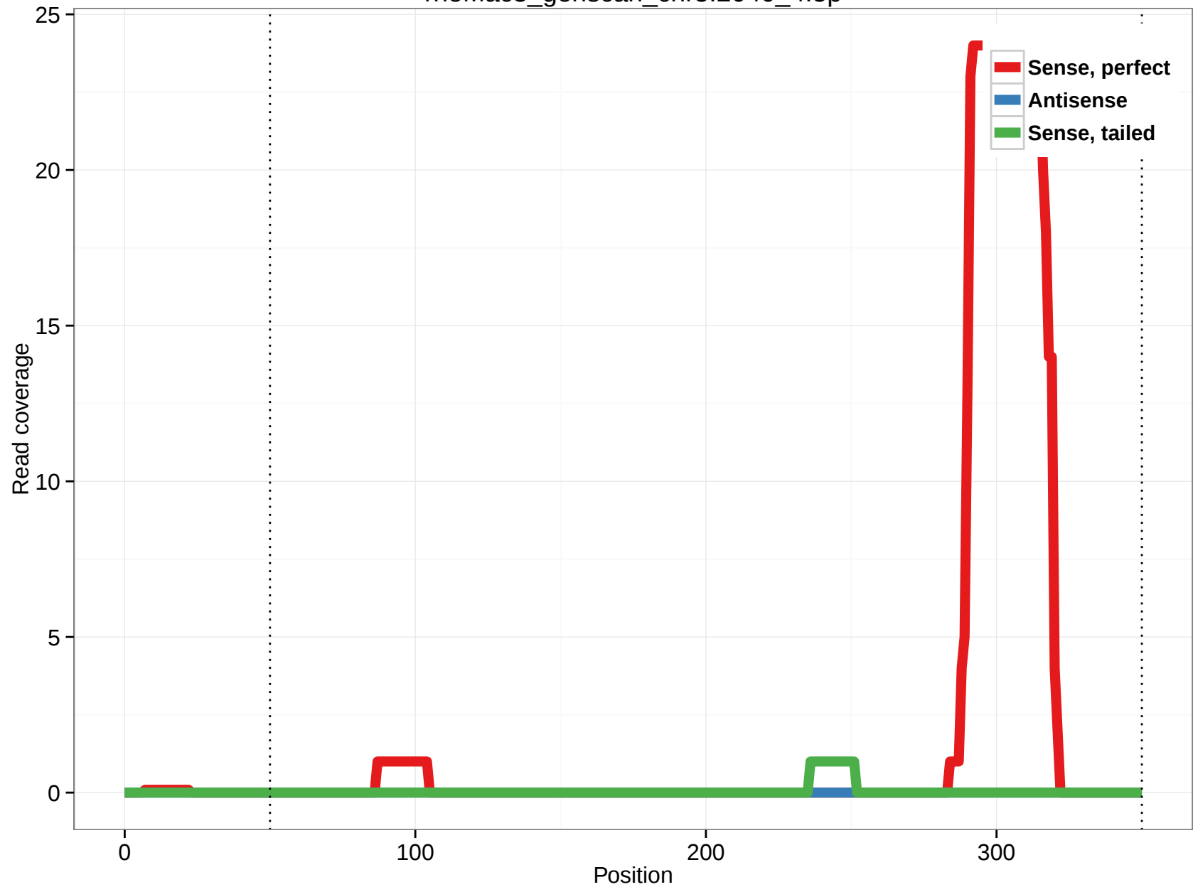
rheMac3_genscan_chr5.2040_4.5p
