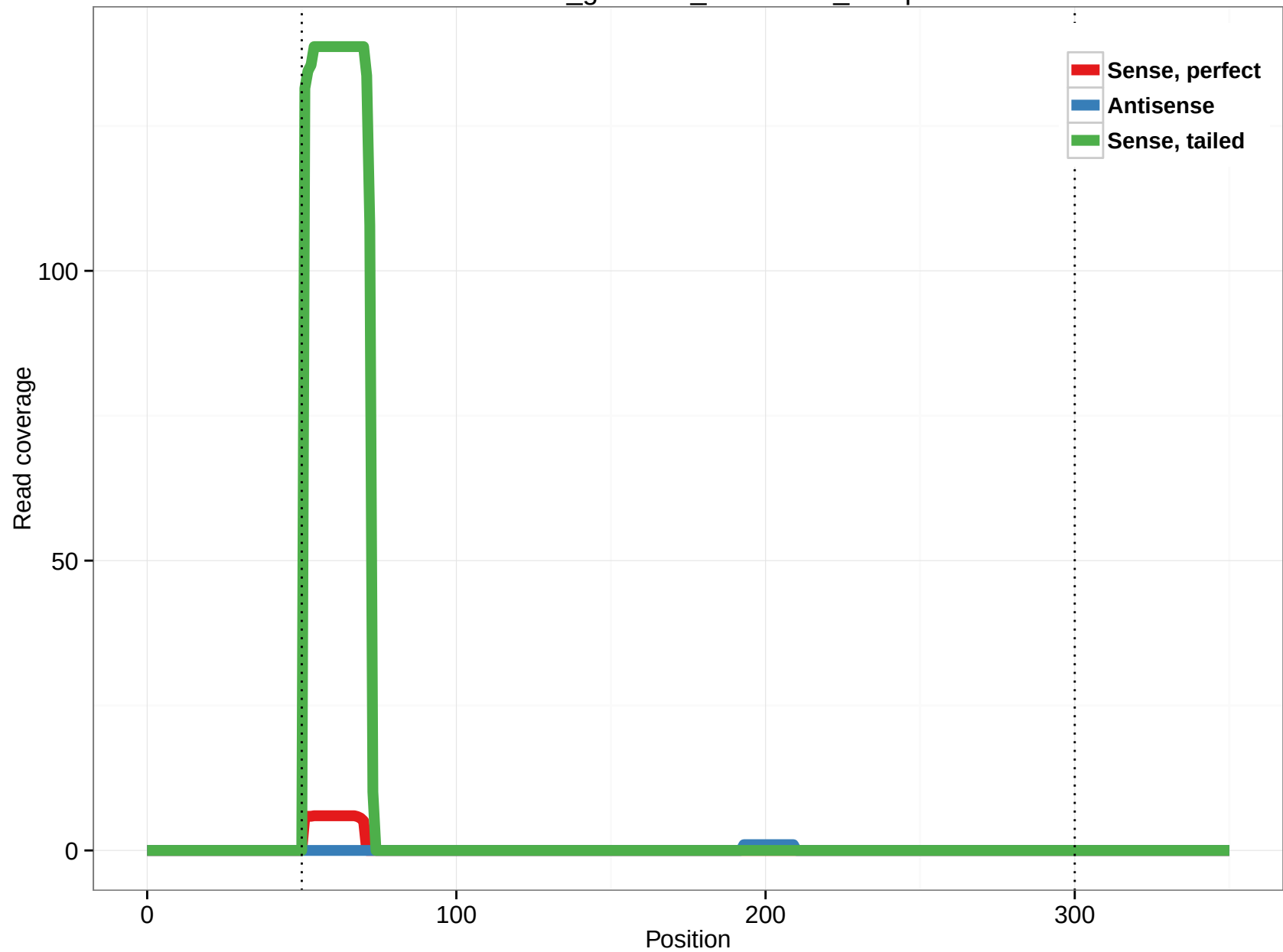
rheMac3_genscan_chr5.1998_11.5p
