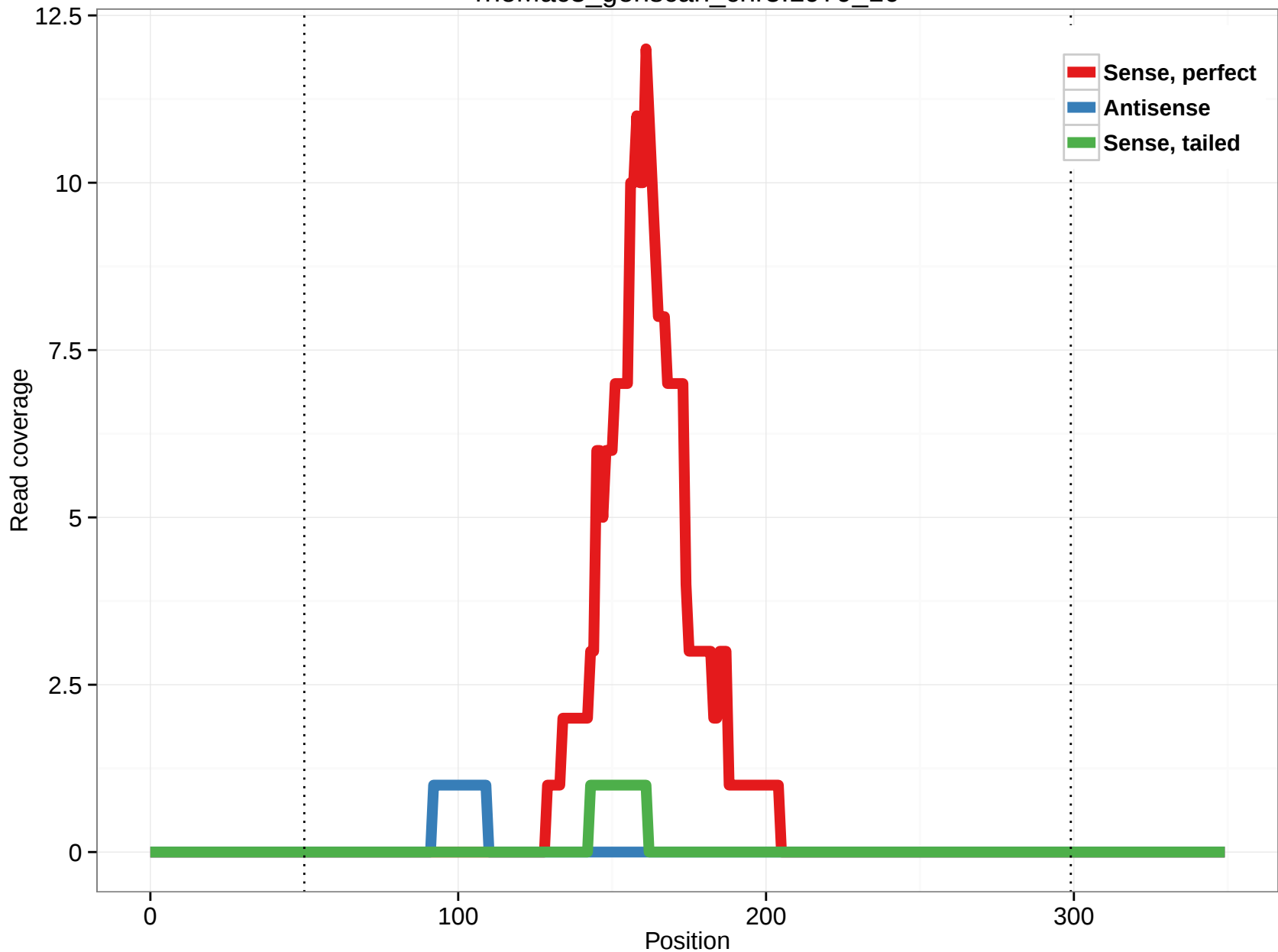
rheMac3_genscan_chr5.1979_10
