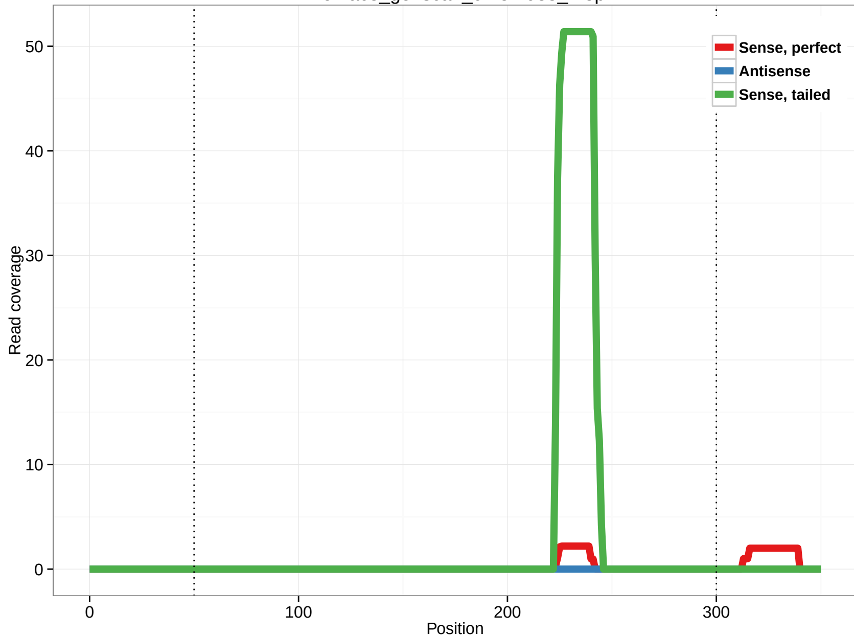
rheMac3_genscan_chr5.1938_7.3p
