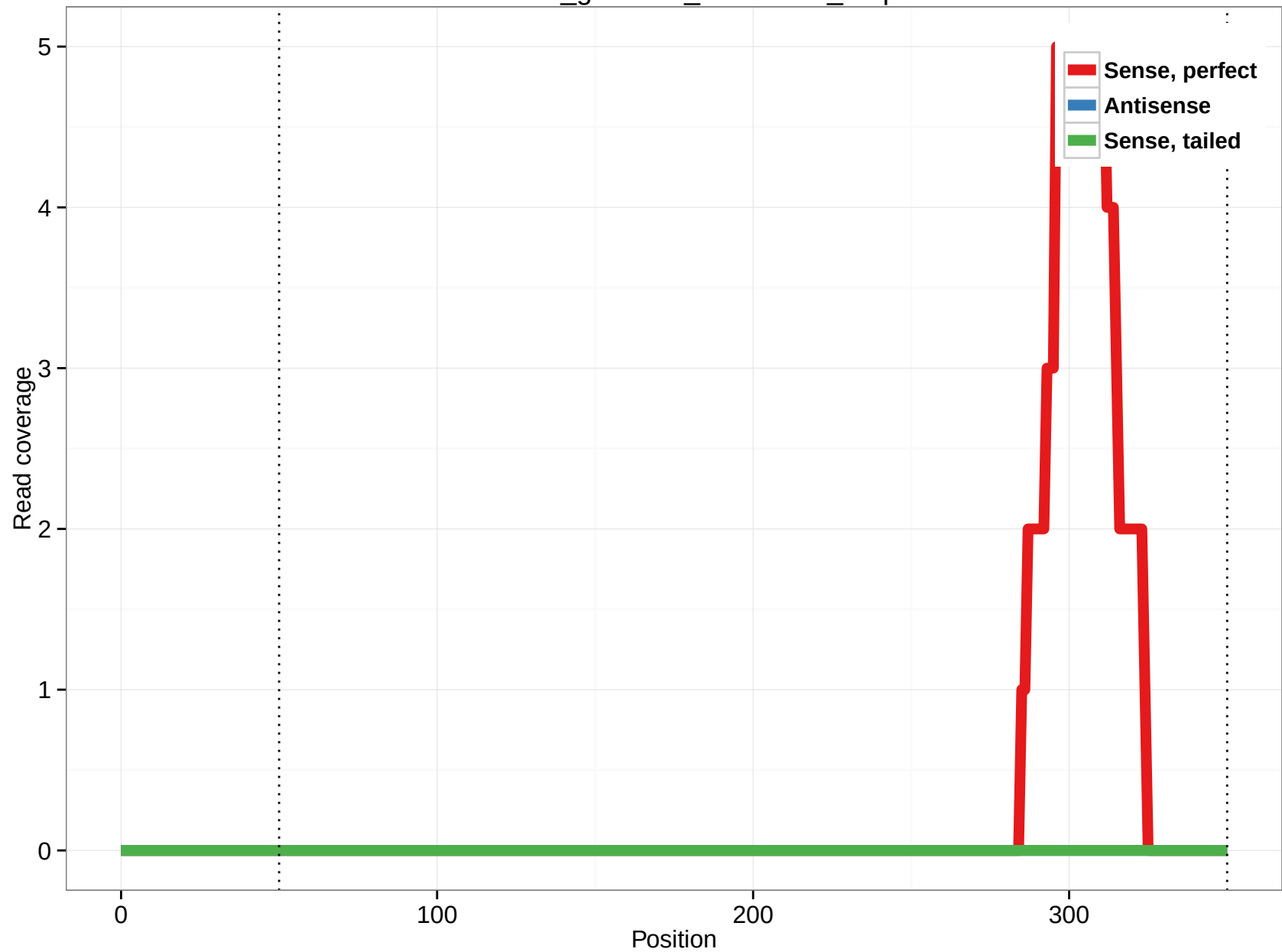
rheMac3_genscan_chr5.1921_5.5p
