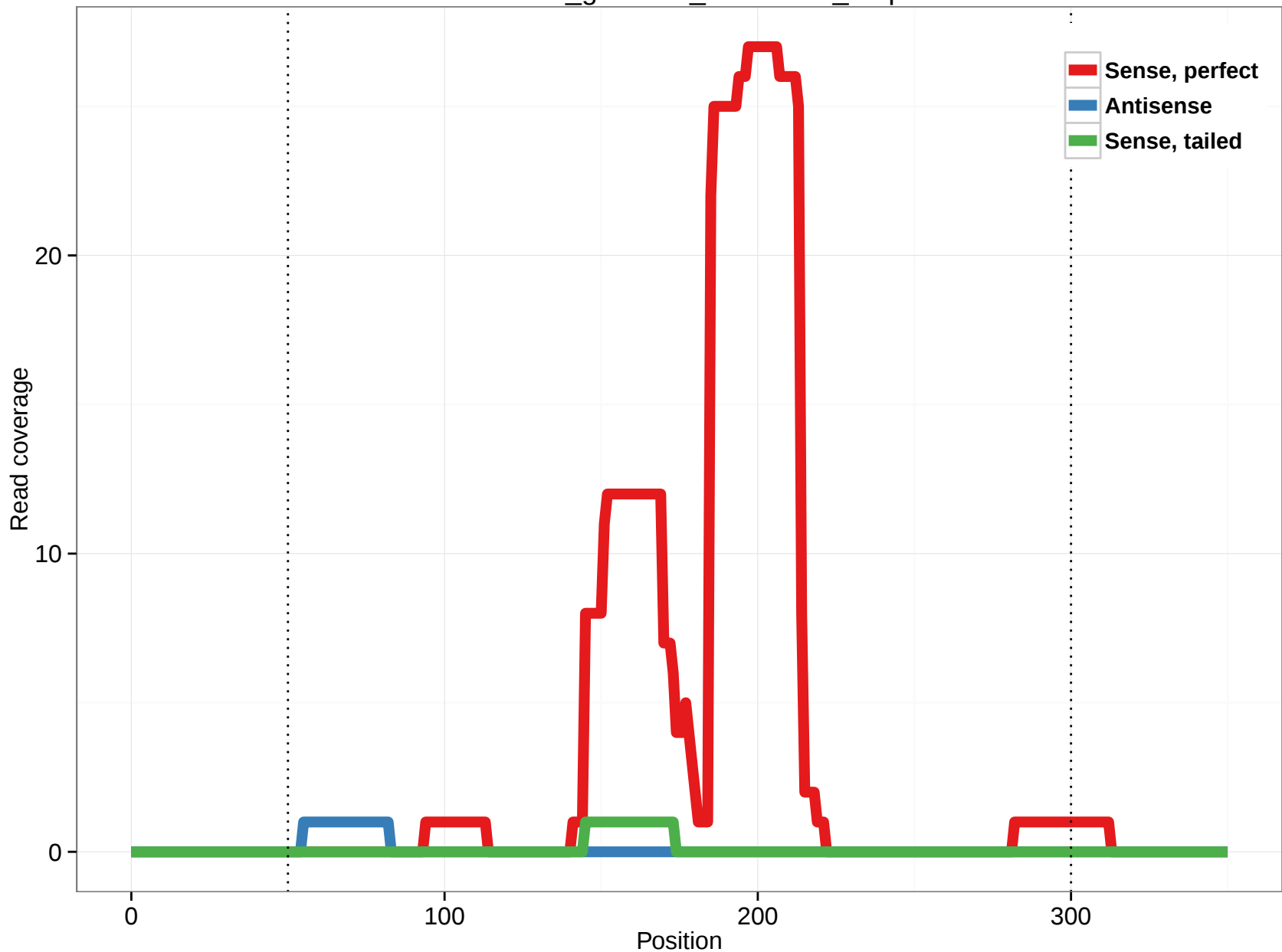
rheMac3_genscan_chr5.1921_4.3p
