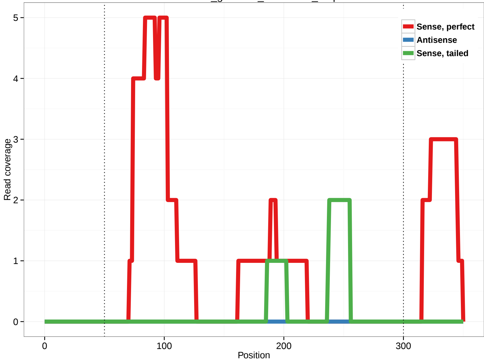
rheMac3_genscan_chr5.1793_7.5p
