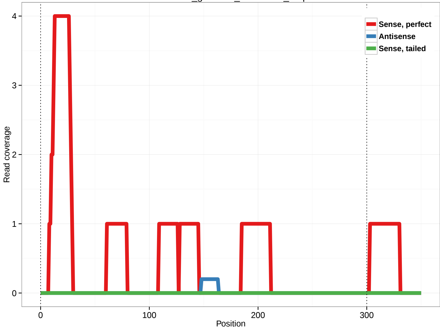
rheMac3_genscan_chr5.1669_6.3p
