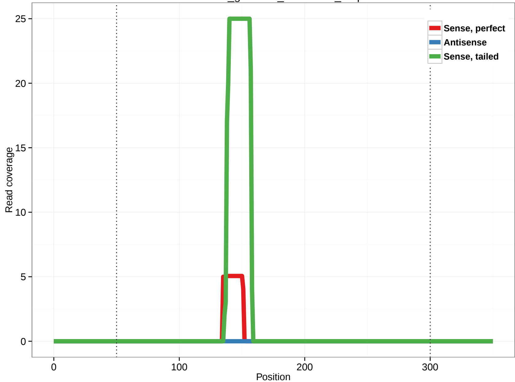
rheMac3_genscan_chr5.1552_3.5p
