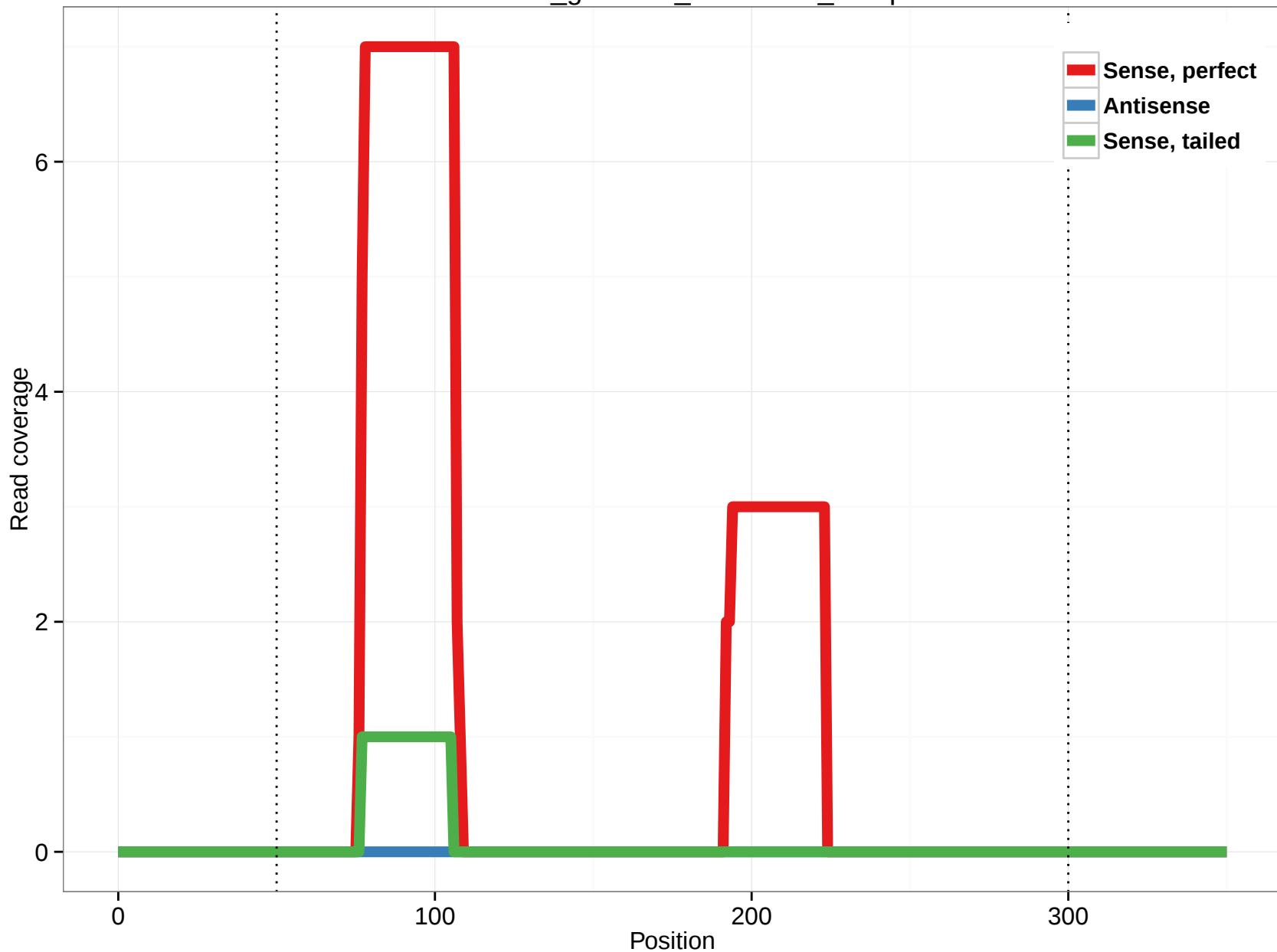
rheMac3_genscan_chr5.1547_11.5p
