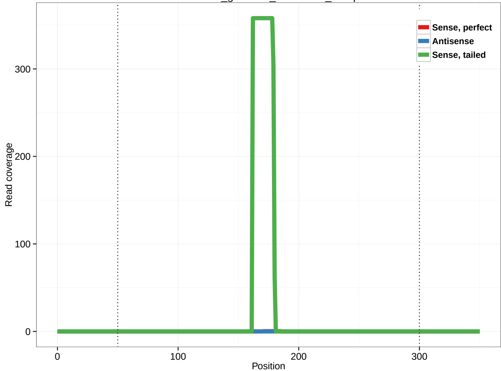
rheMac3_genscan_chr5.1448_13.5p
