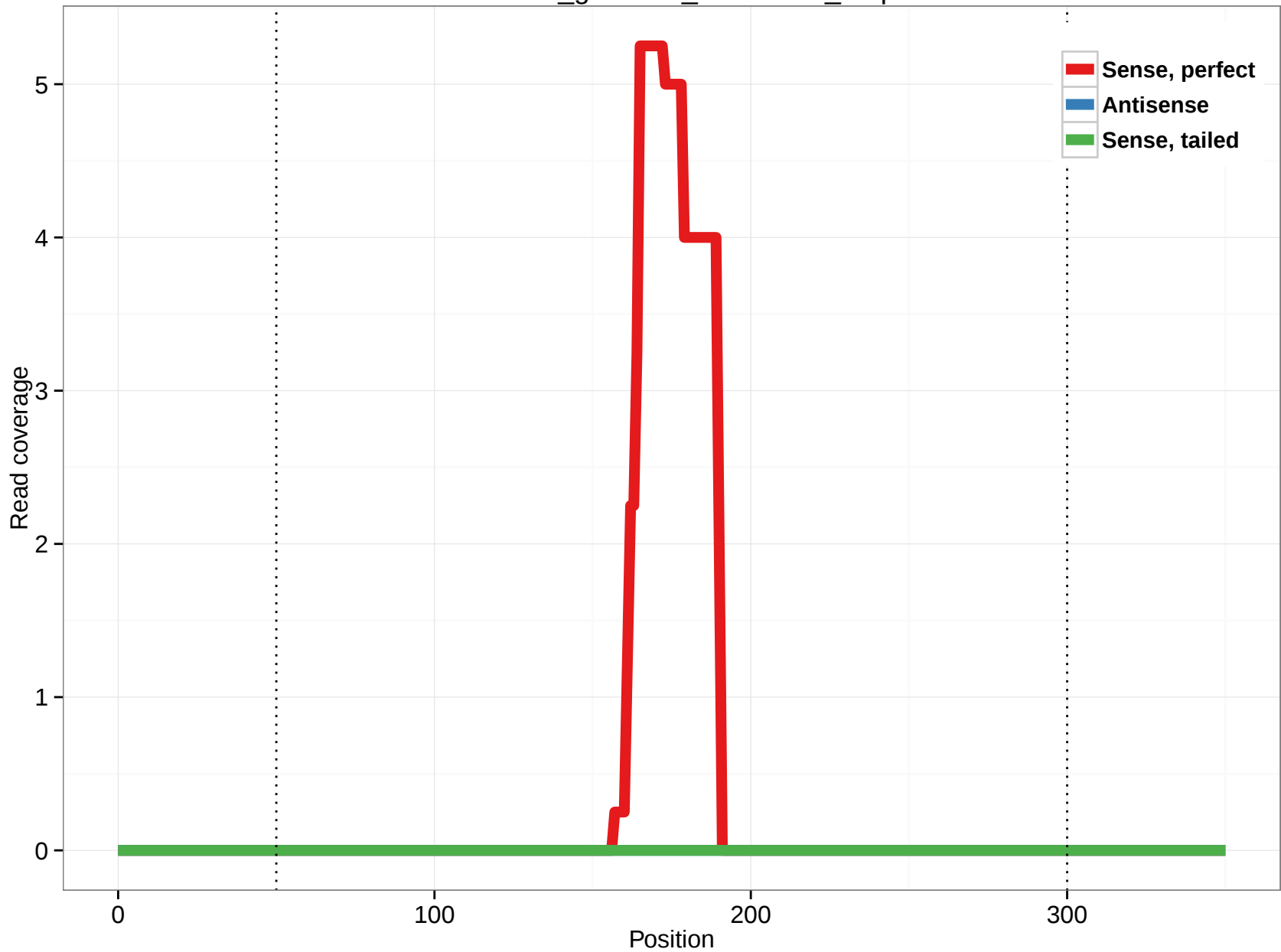
rheMac3_genscan_chr5.1370_0.5p
