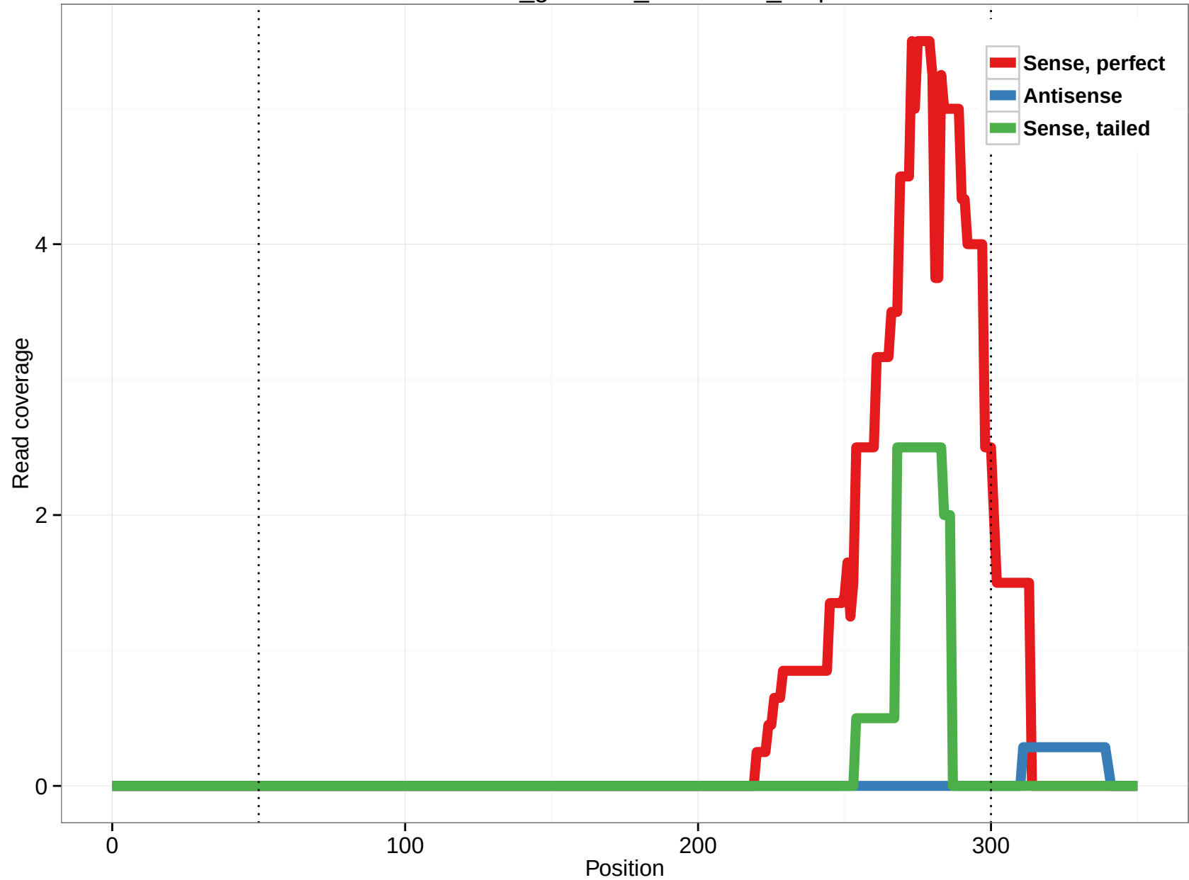
rheMac3_genscan_chr5.1311_5.3p
