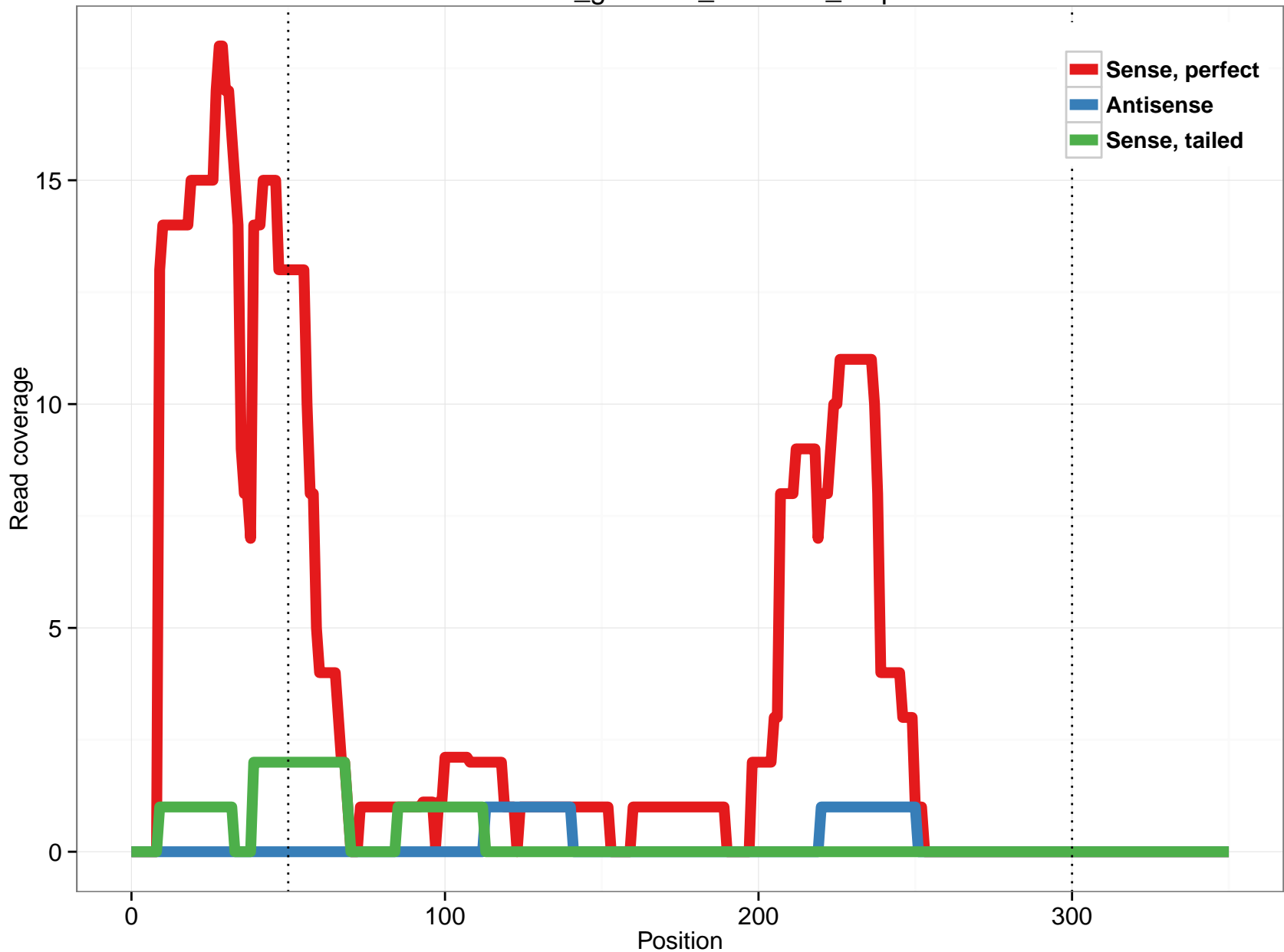
rheMac3_genscan_chr5.123_1.5p
