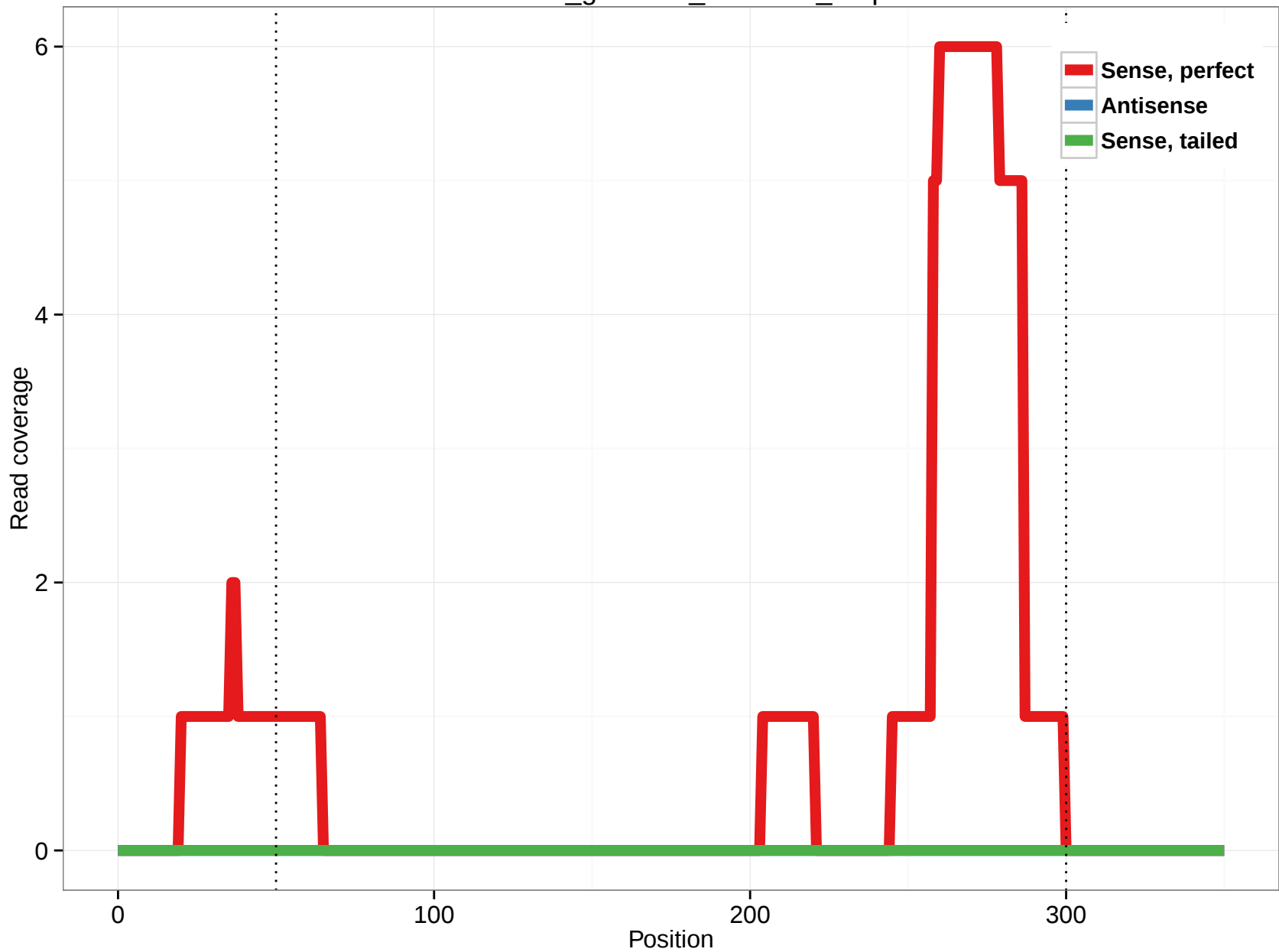
rheMac3_genscan_chr5.123_0.5p
