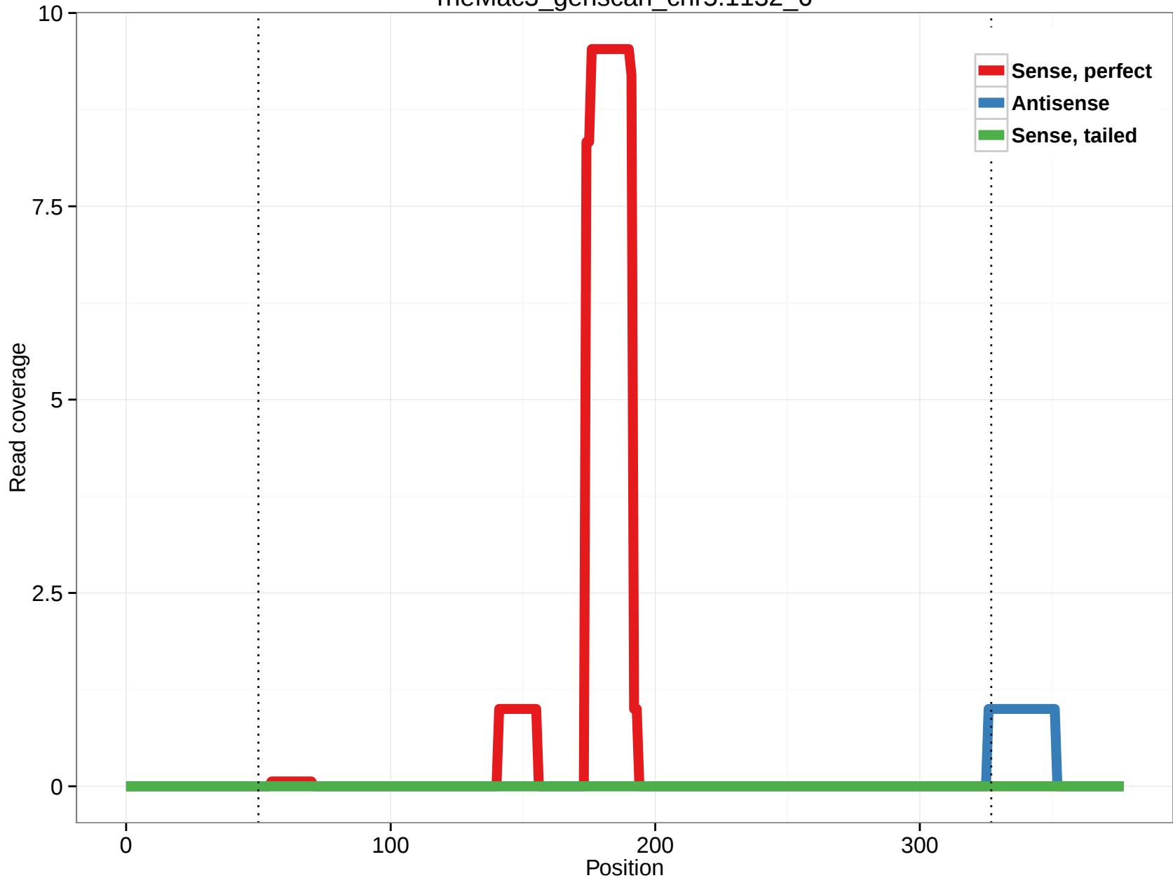
rheMac3_genscan_chr5.1132_6
