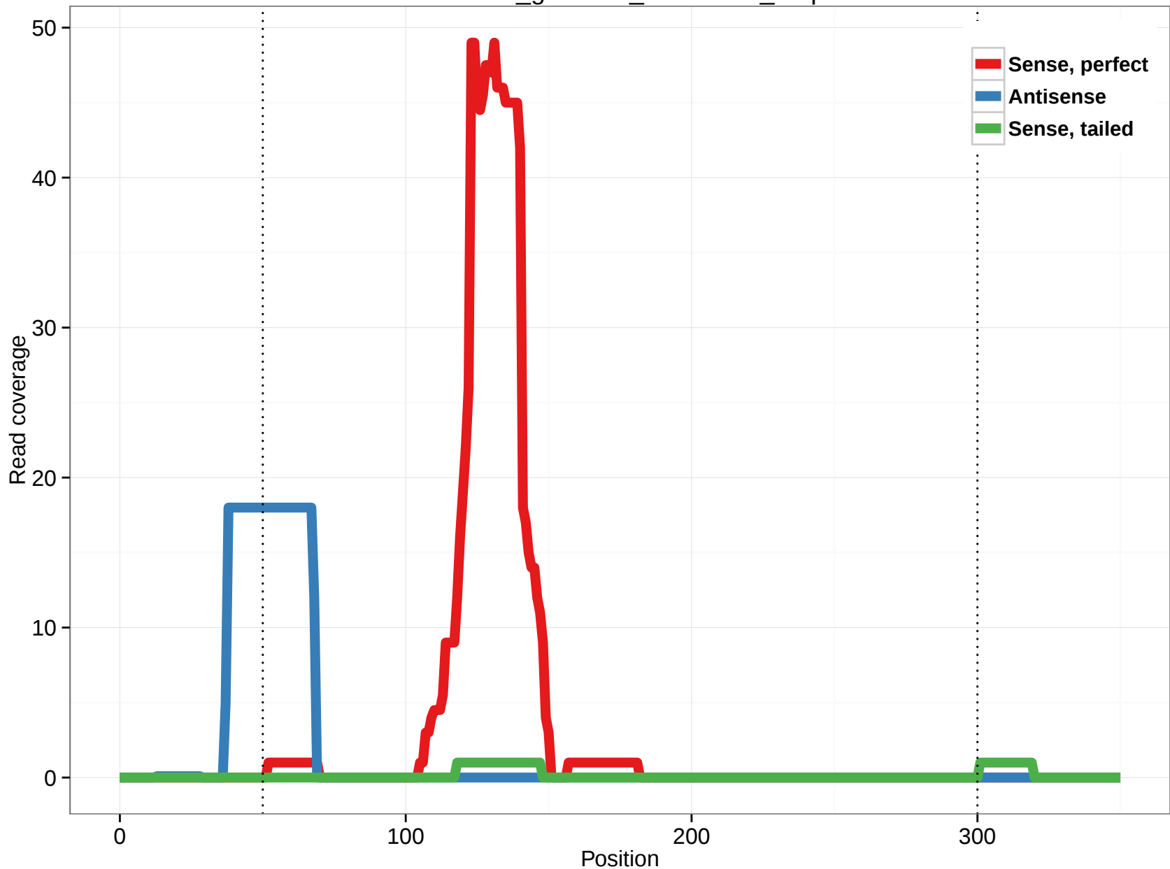
rheMac3_genscan_chr5.1124_0.5p
