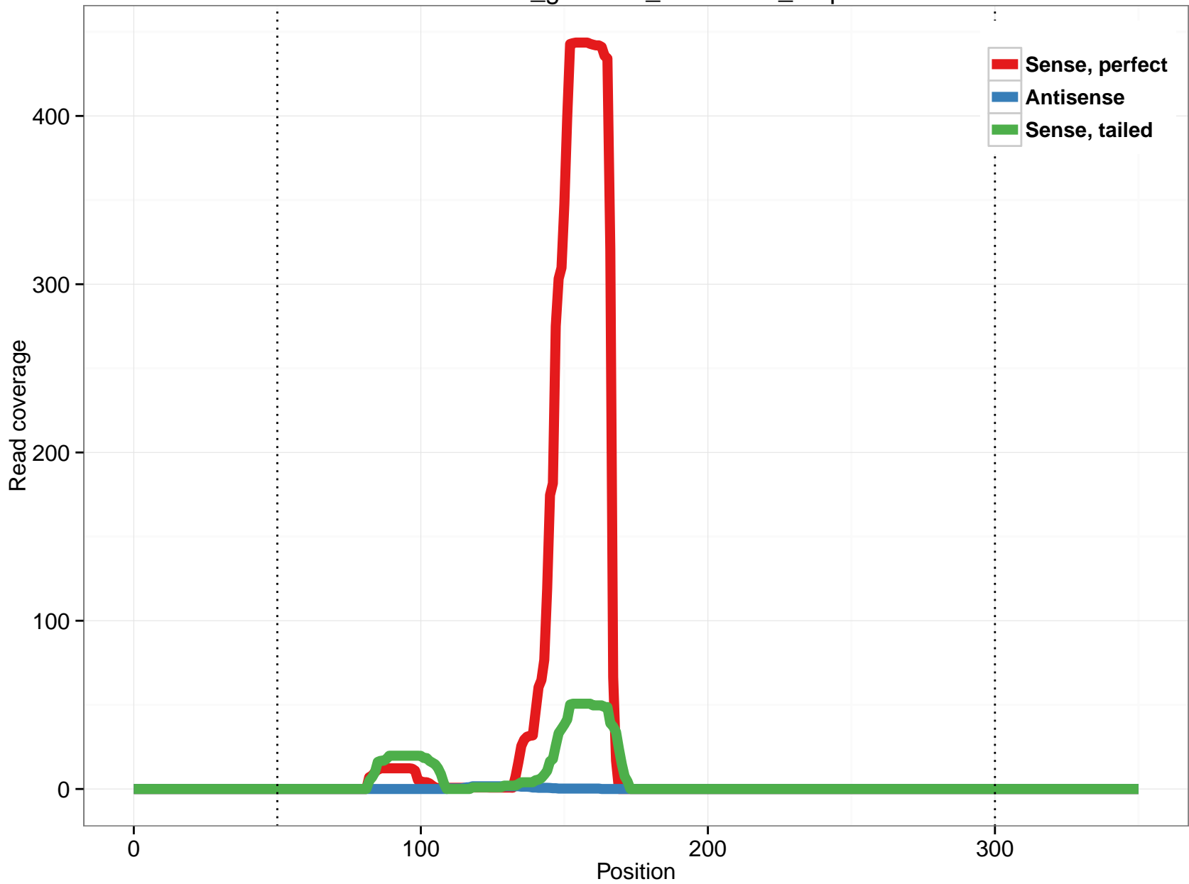
rheMac3_genscan_chr5.1046_0.5p
