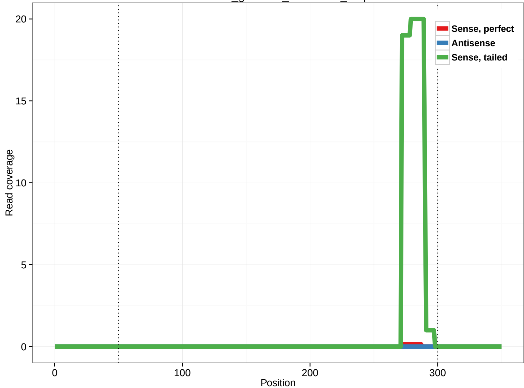
rheMac3_genscan_chr5.1038_6.5p
