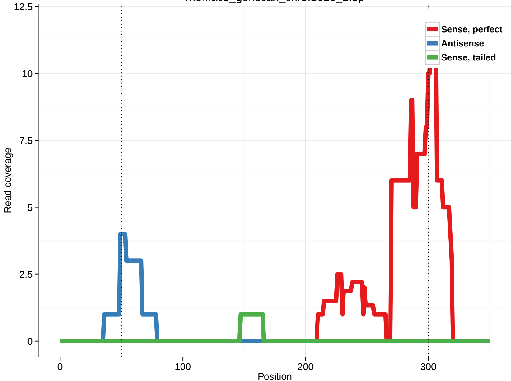
rheMac3_genscan_chr5.1026_1.3p
