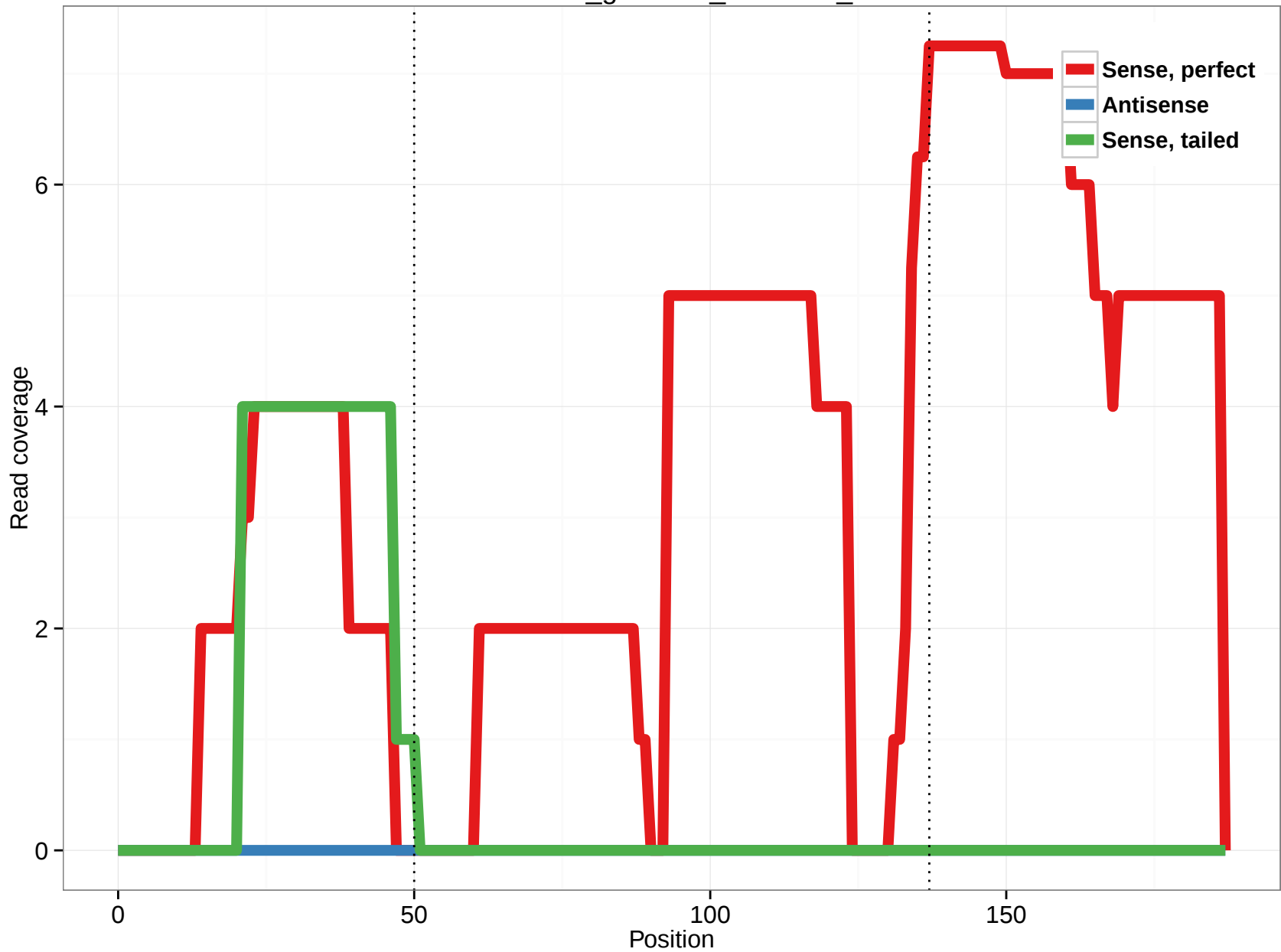
rheMac3_genscan_chr5.101_5
