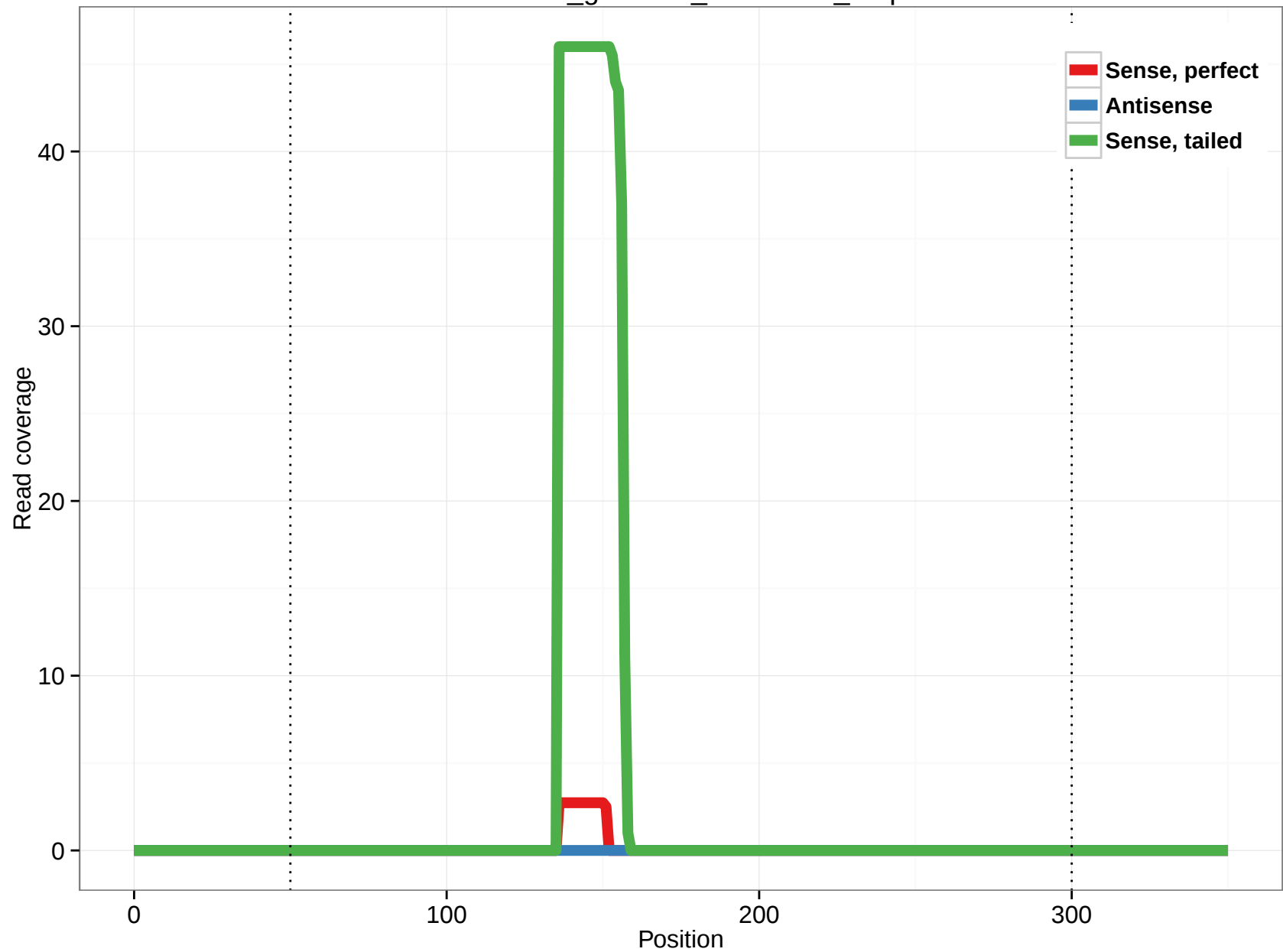
rheMac3_genscan_chr5.1001_2.3p
