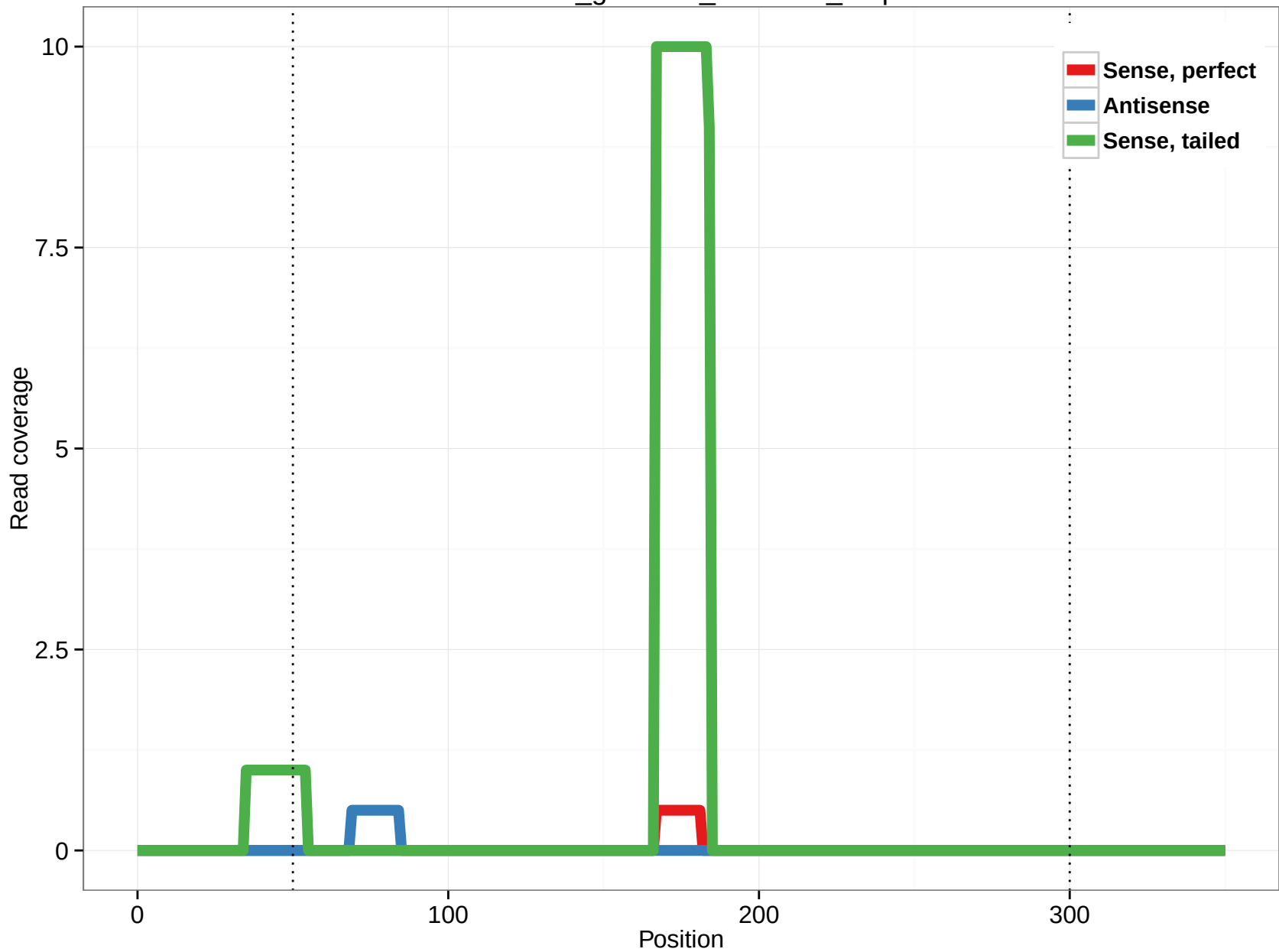
rheMac3_genscan_chr4.995_0.5p
