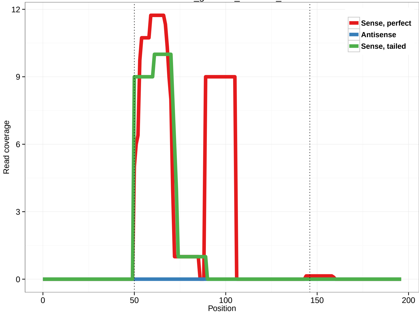
rheMac3_genscan_chr4.992_5
