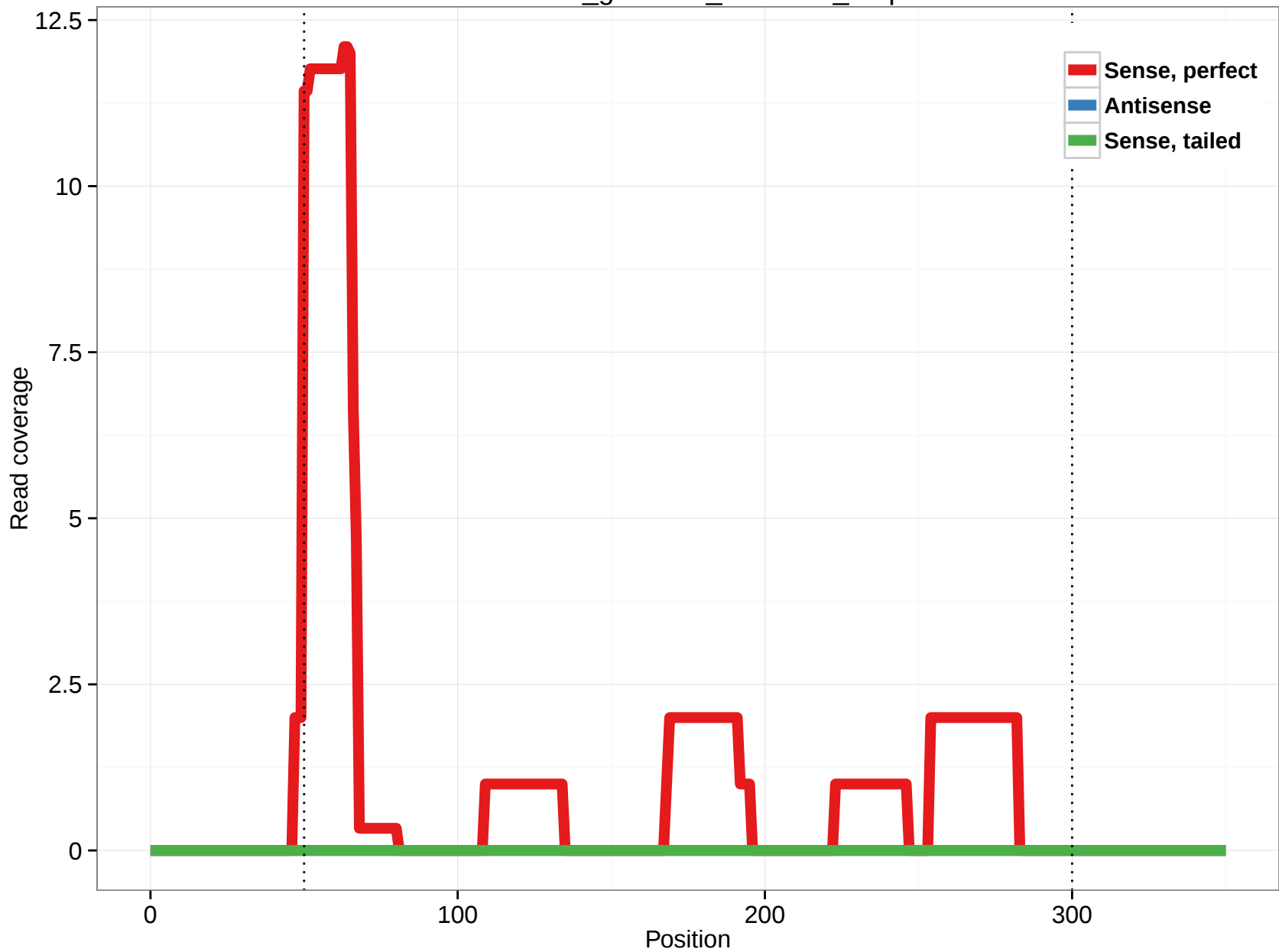
rheMac3_genscan_chr4.989_3.5p
