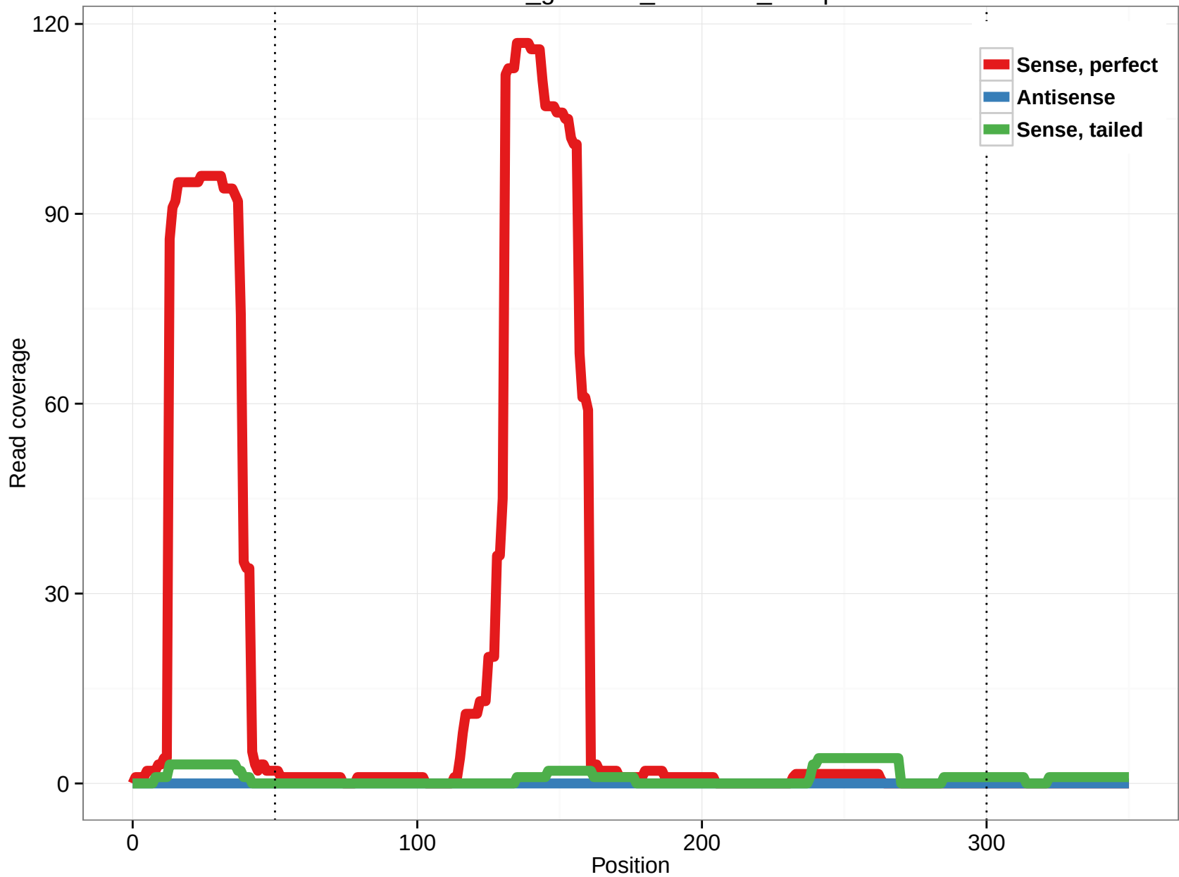
rheMac3_genscan_chr4.985_32.5p
