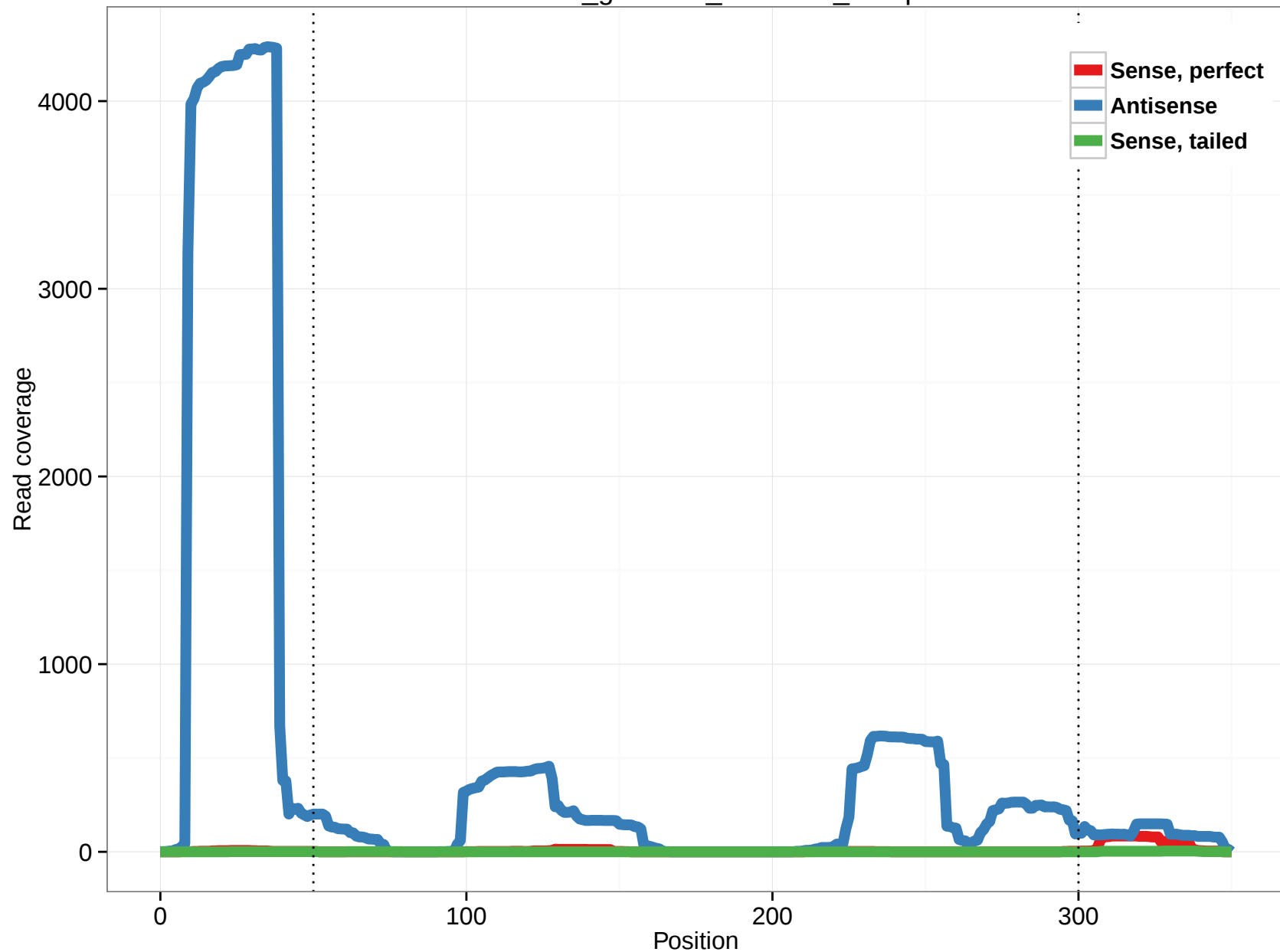
rheMac3_genscan_chr4.985_27.3p
