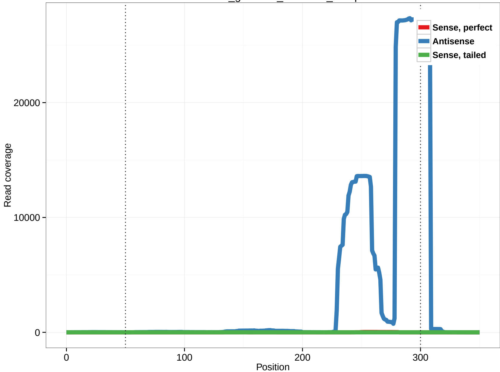
rheMac3_genscan_chr4.985_26.3p
