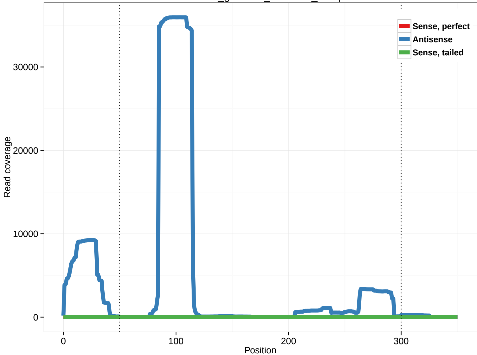
rheMac3_genscan_chr4.985_25.3p
