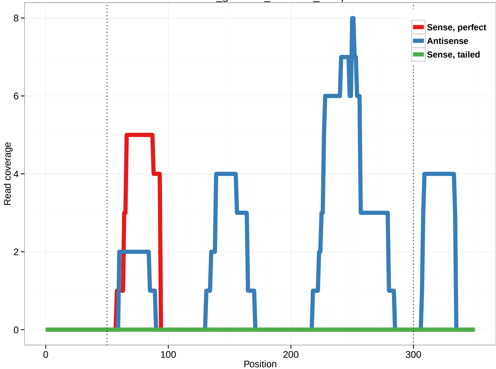
rheMac3_genscan_chr4.985_21.3p
