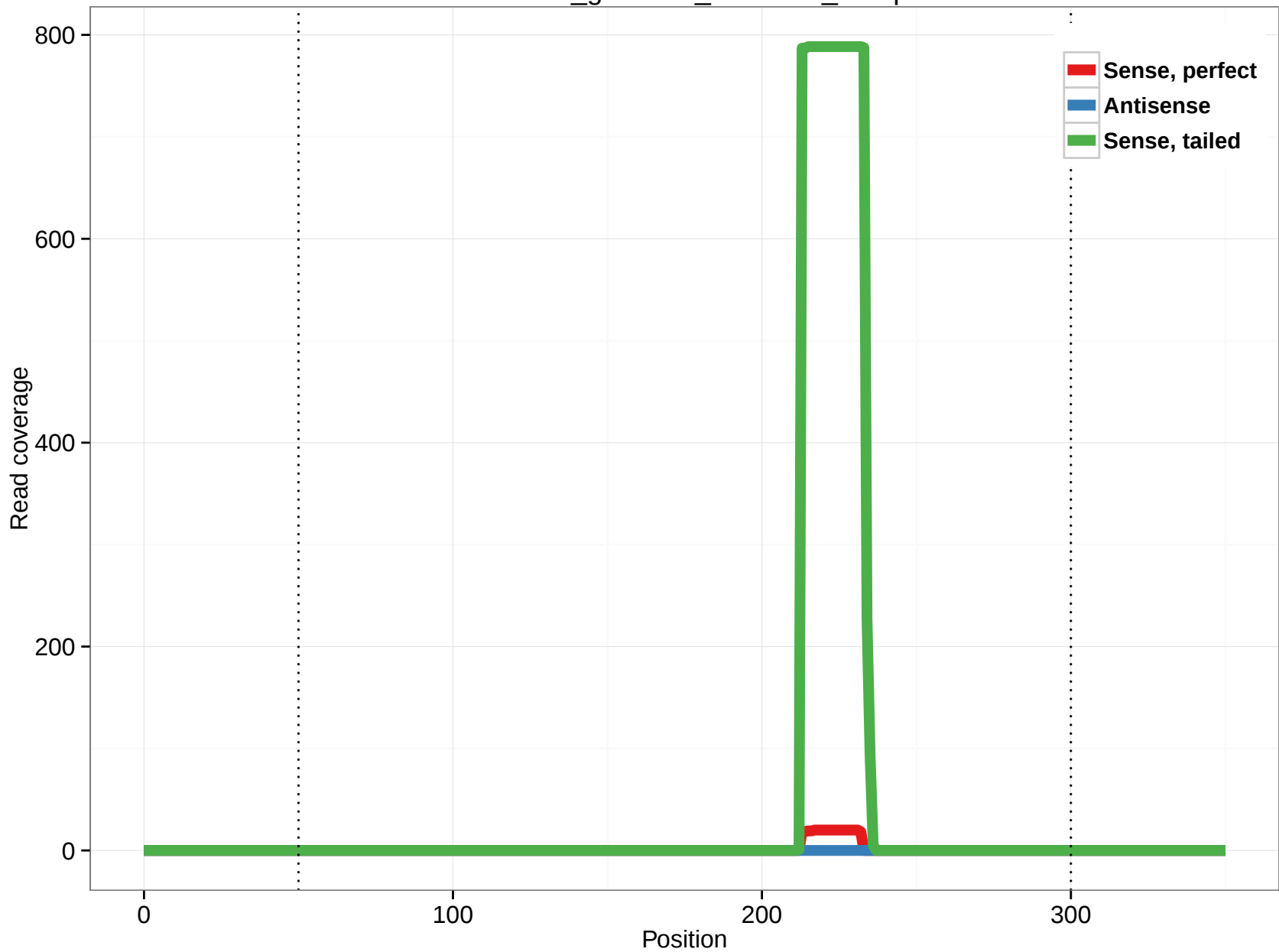
rheMac3_genscan_chr4.970_57.5p
