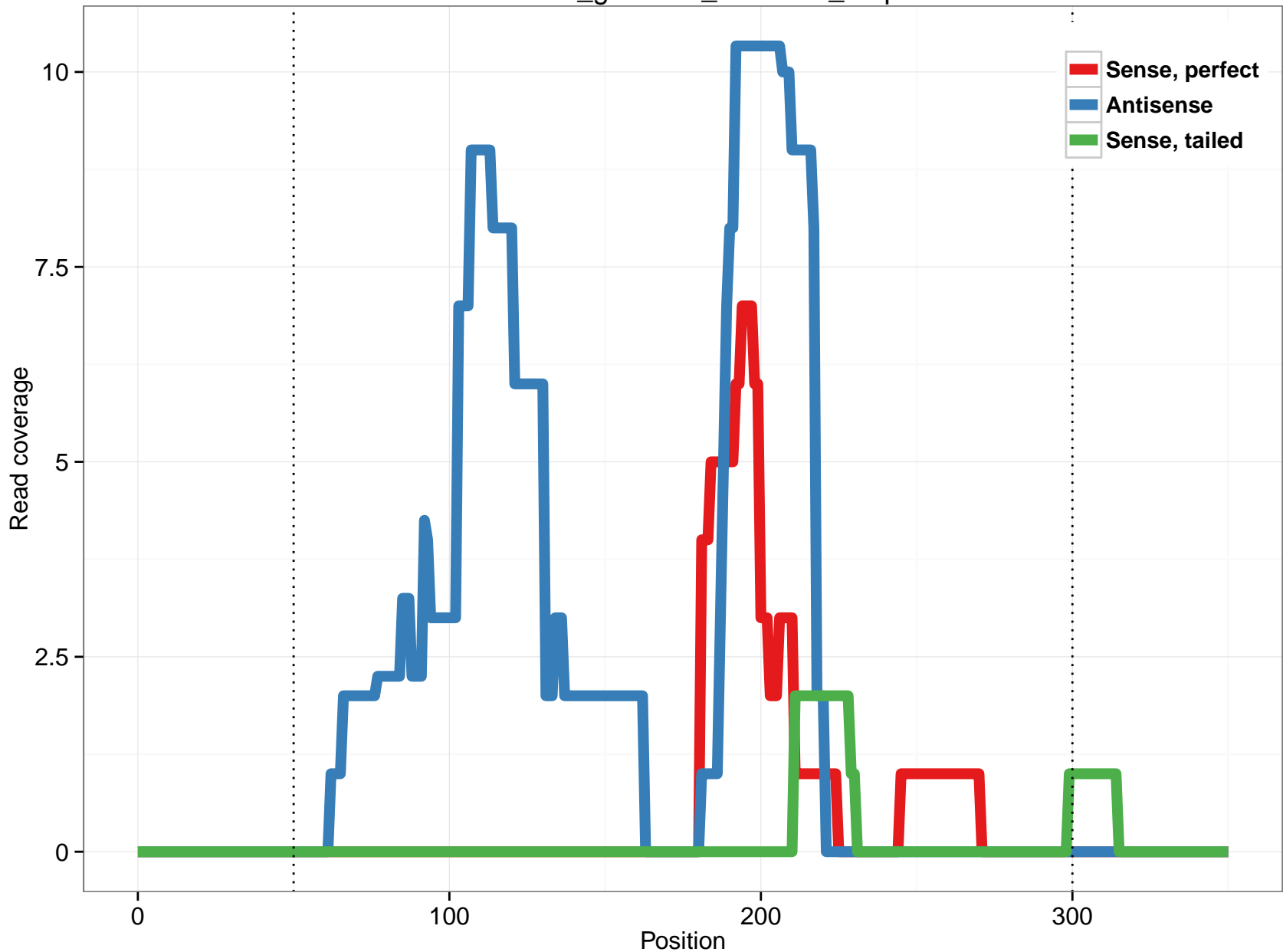
rheMac3_genscan_chr4.969_2.5p
