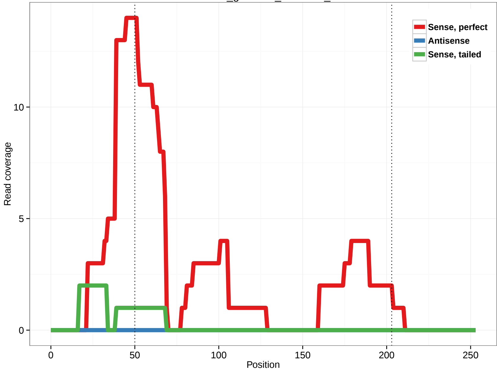
rheMac3_genscan_chr4.966_22
