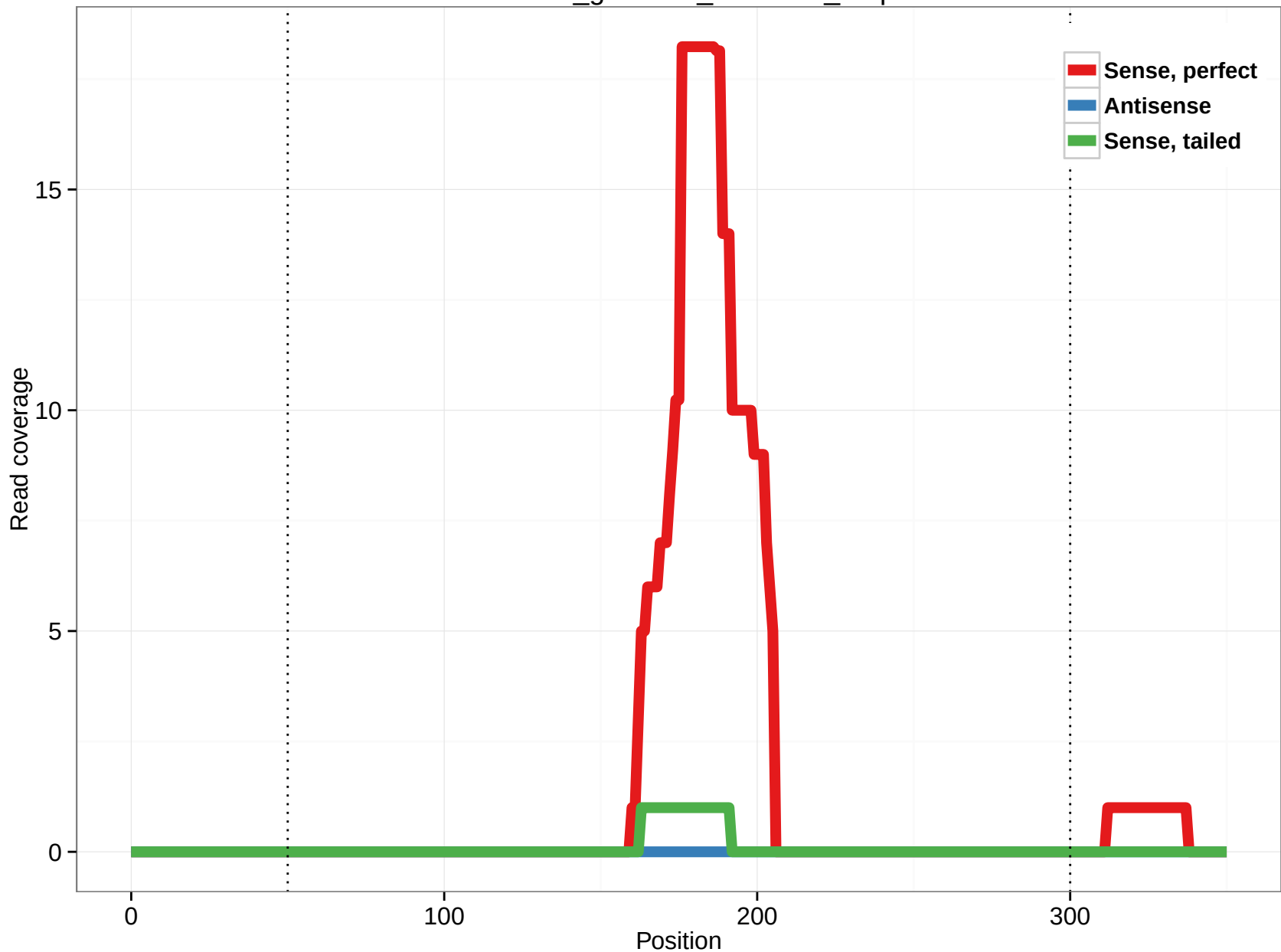
rheMac3_genscan_chr4.964_9.3p
