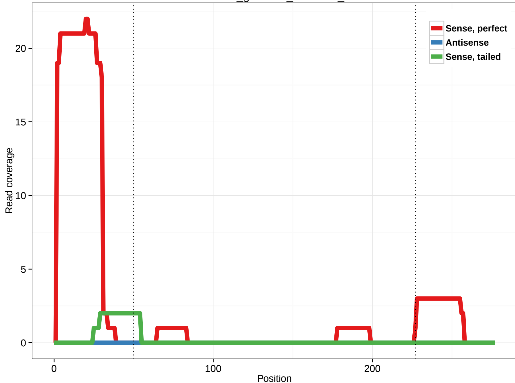
rheMac3_genscan_chr4.964_13
