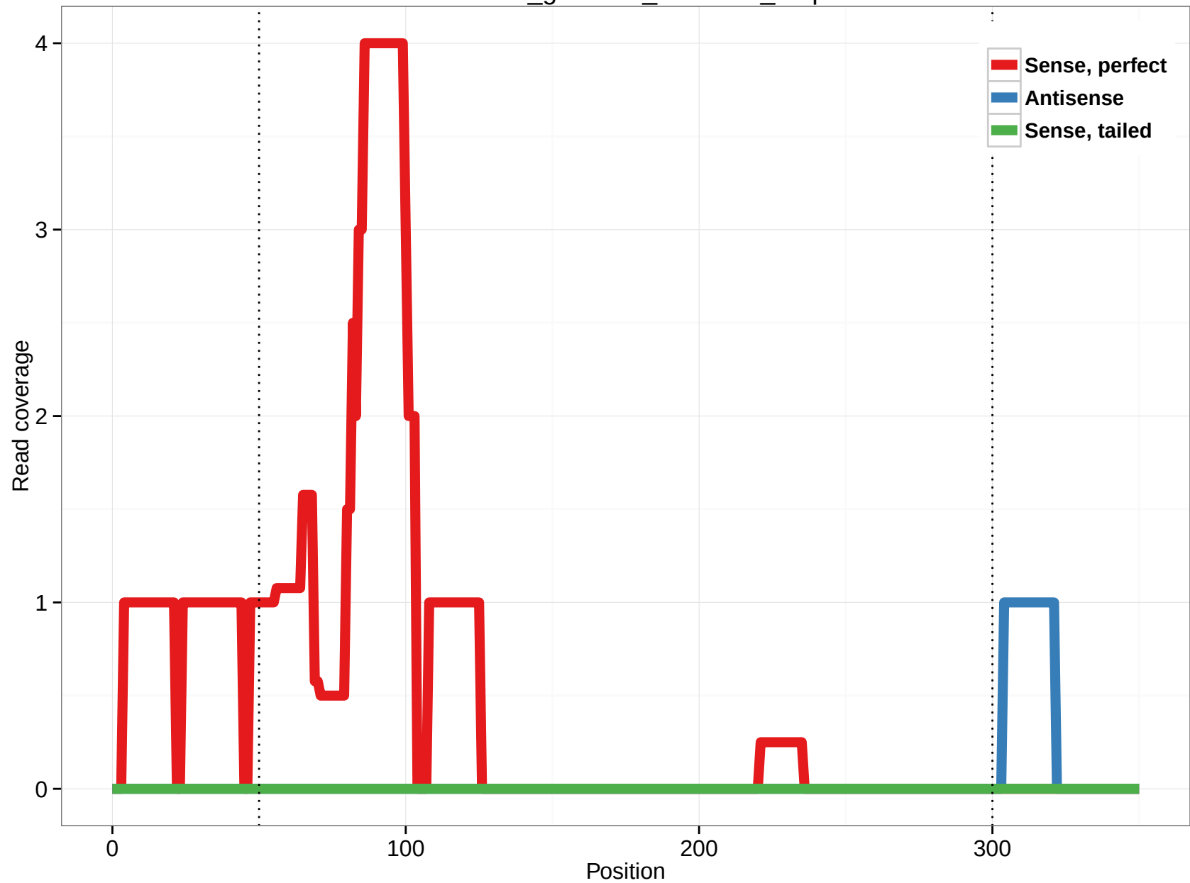
rheMac3_genscan_chr4.963_2.5p
