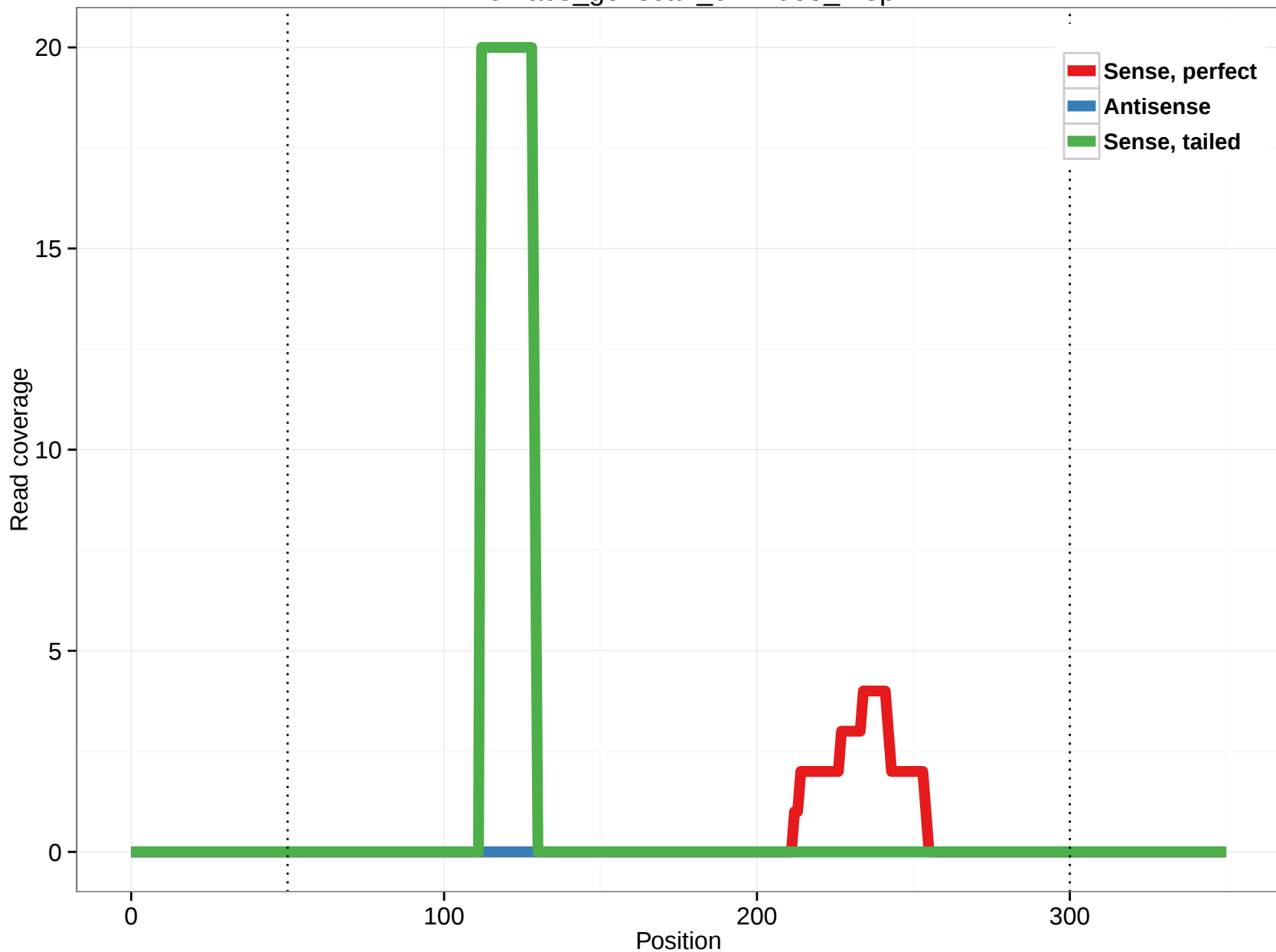
rheMac3_genscan_chr4.955_1.5p
