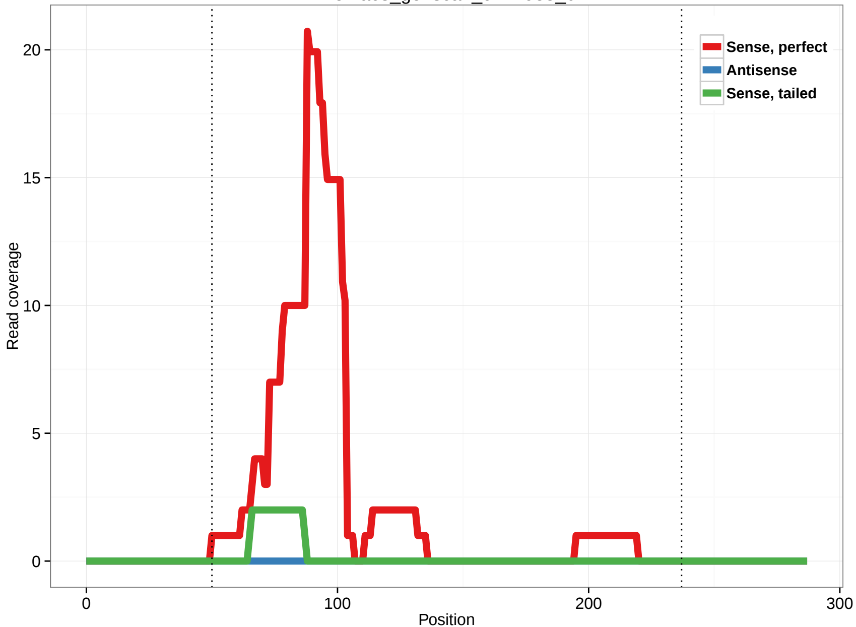
rheMac3_genscan_chr4.955_0
