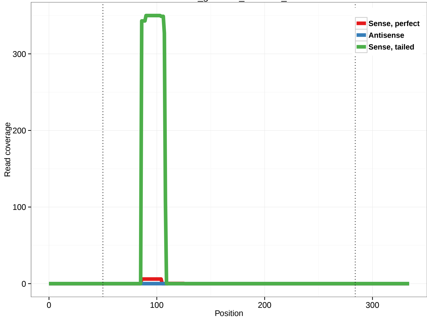
rheMac3_genscan_chr4.953_36
