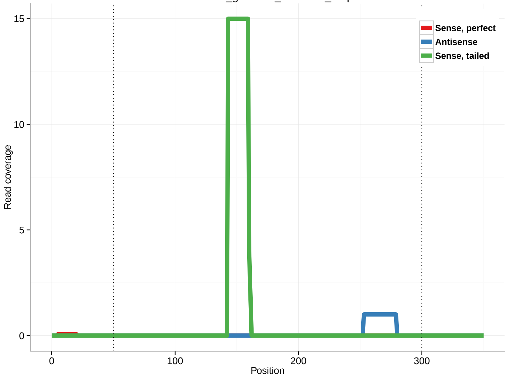
rheMac3_genscan_chr4.952_2.5p
