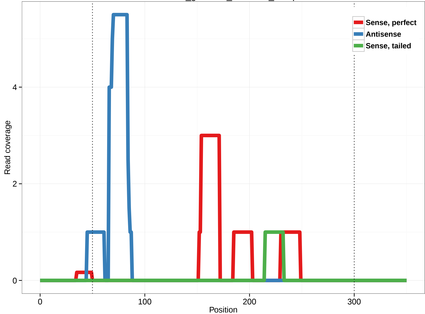
rheMac3_genscan_chr4.934_25.3p
