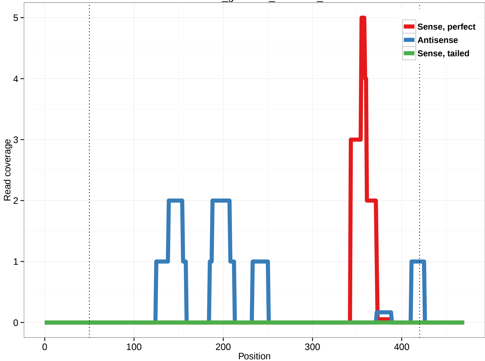
rheMac3_genscan_chr4.877_0
