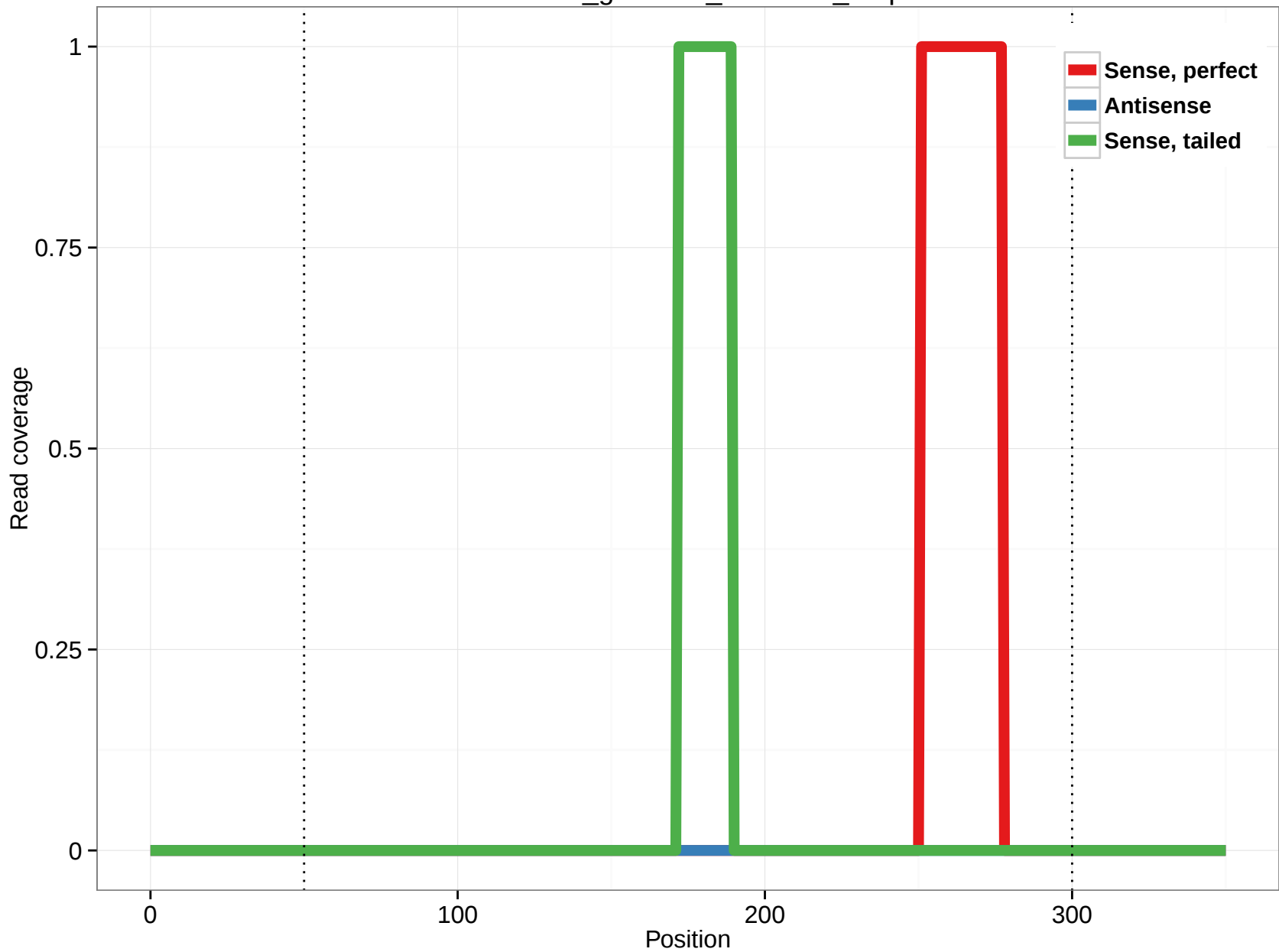
rheMac3_genscan_chr4.870_3.3p
