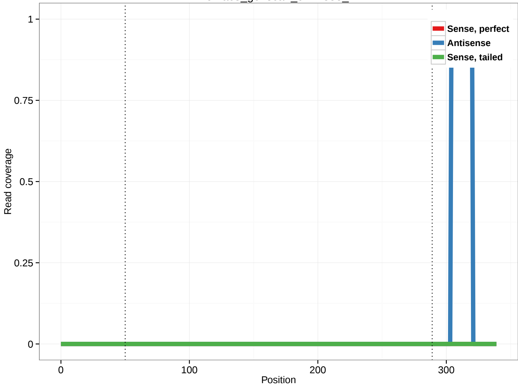
rheMac3_genscan_chr4.858_44
