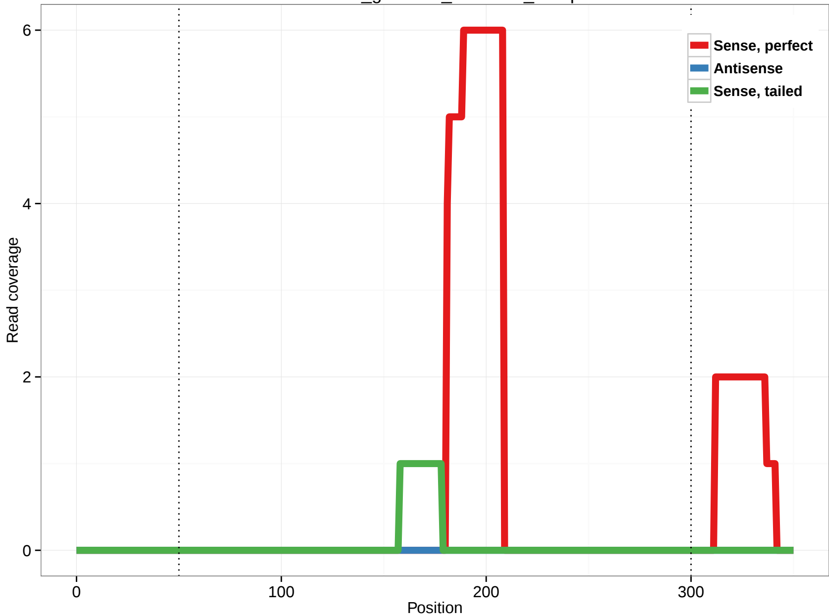
rheMac3_genscan_chr4.852_10.3p
